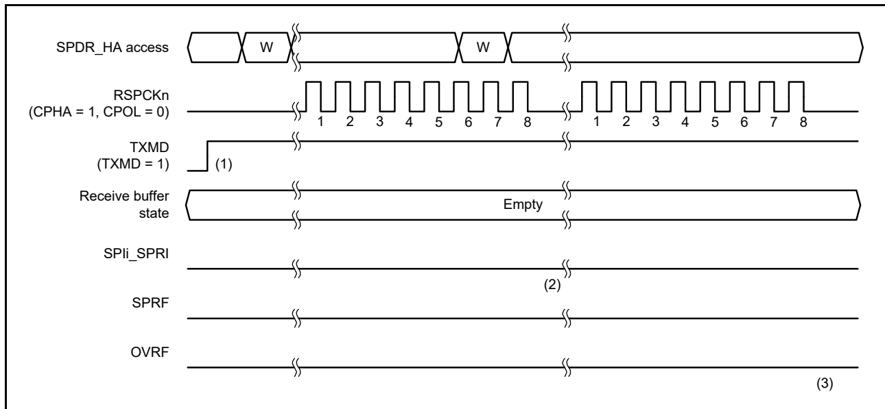
Figure 38.25 Operation example when SPCR.TXMD = 1
