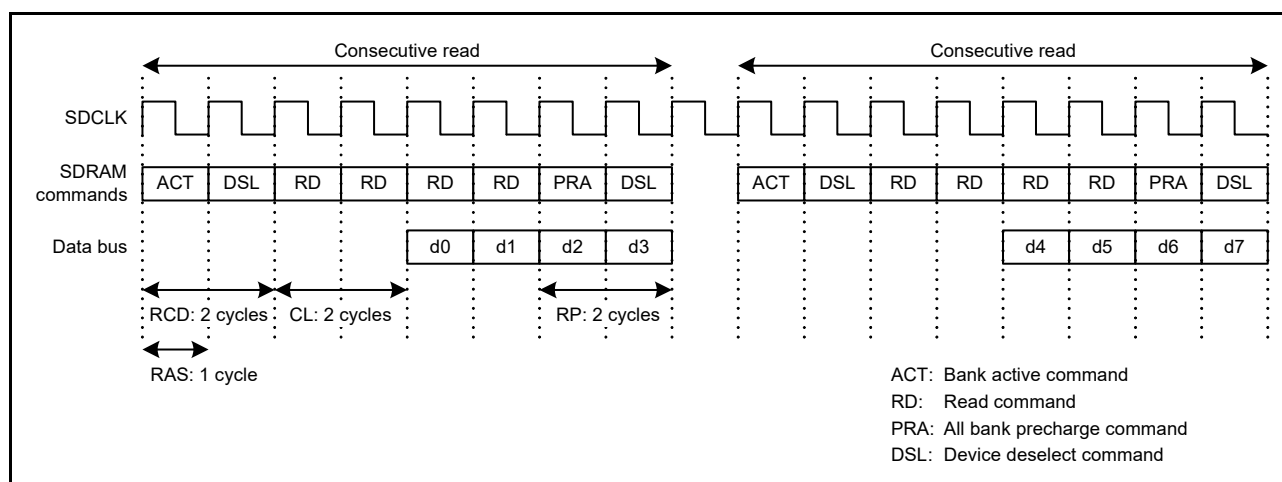
Figure 15.65 Example timing for consecutive read (2)
