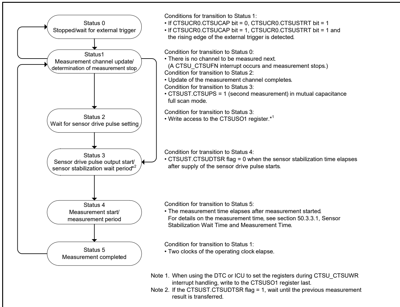
Figure 51.11 Status operation transitions
