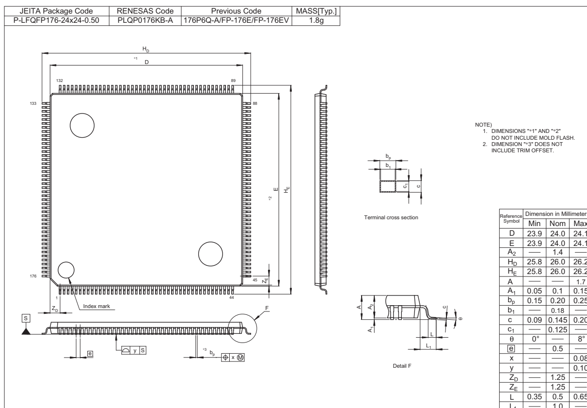
Figure 2.2 176-pin LQFP
