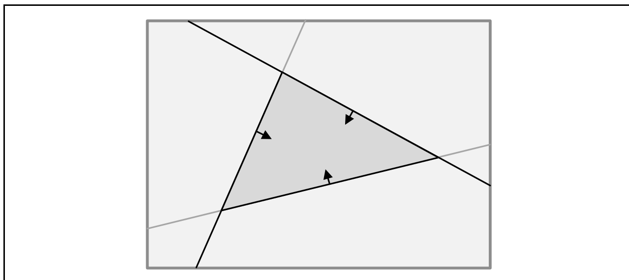
Figure 56.5 Intersection of half planes
