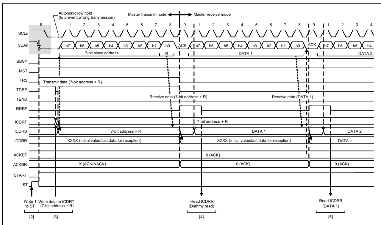
Figure 36.12 Master receive operation timing (1) with 7-bit address format, when RDRFS = 0
