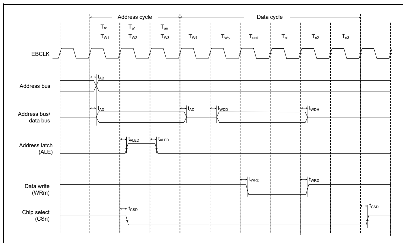
Figure 60.21 Address/data multiplexed bus write access timing
