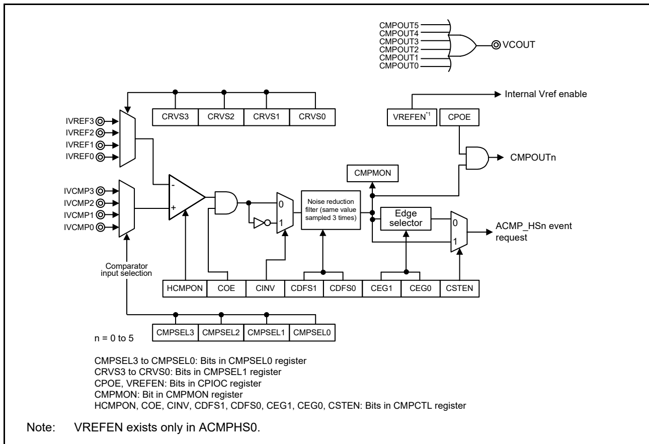
Figure 50.1 ACMPHS block diagram
