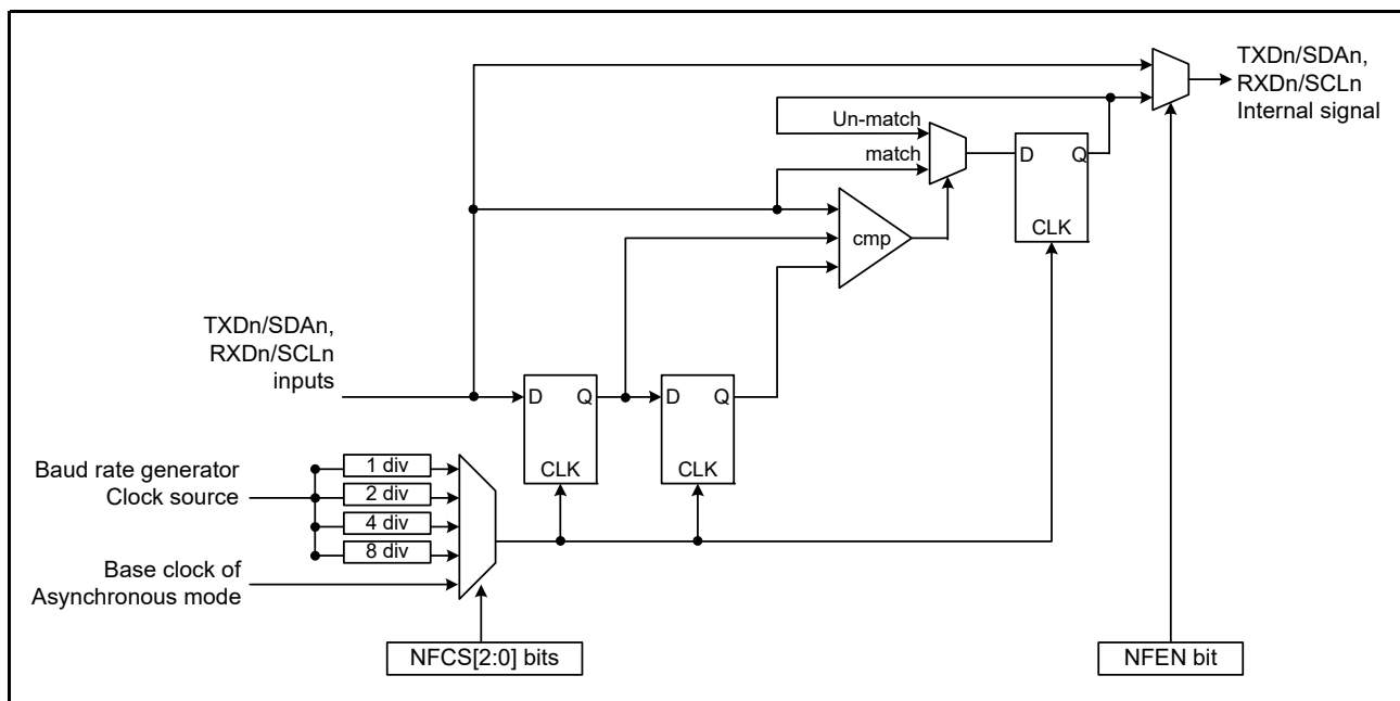
Figure 34.72 Digital noise filter circuit block diagram
