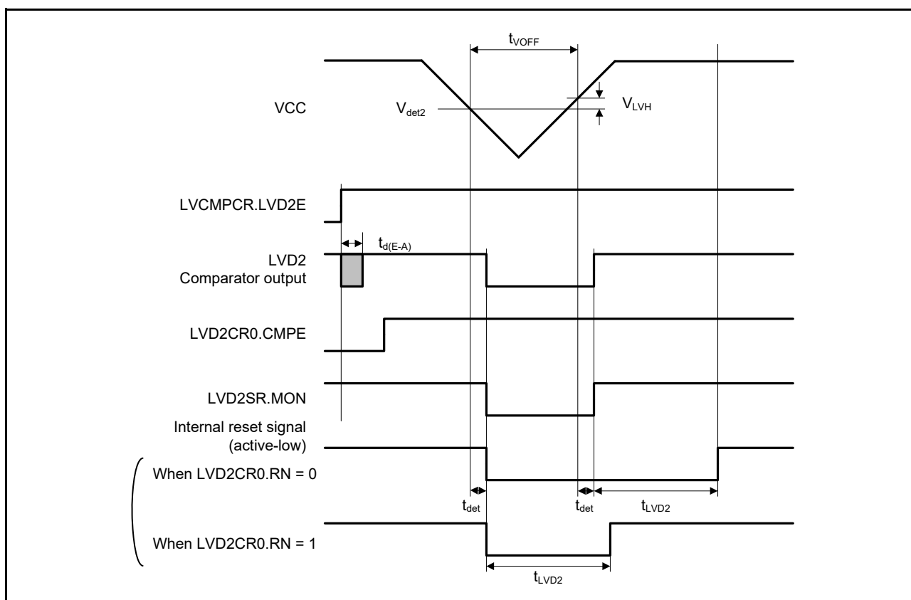
Figure 60.100 Voltage detection circuit timing ( V_{det2} )
