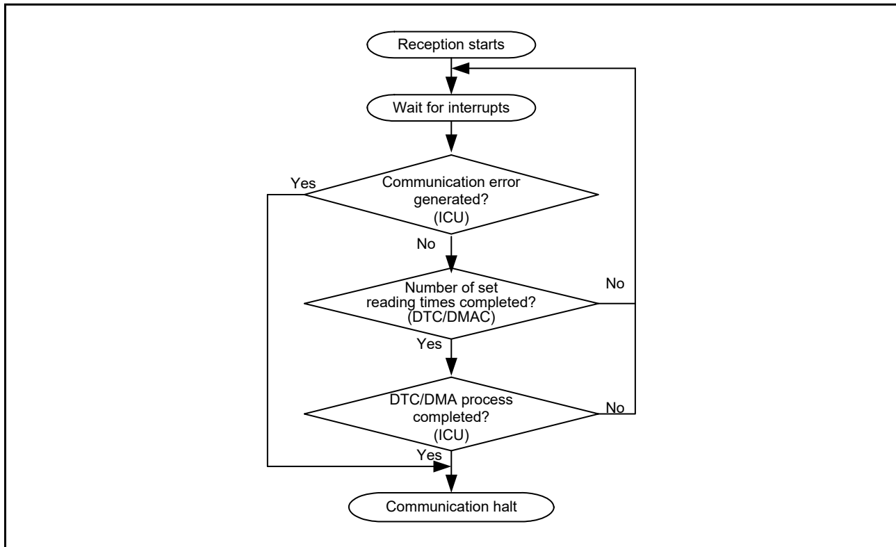
Figure 41.55 Reception procedure
