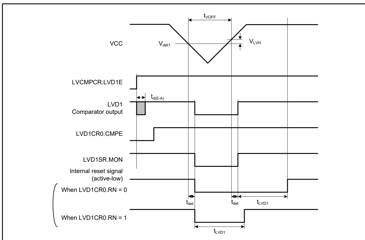
Figure 60.99 Voltage detection circuit timing ( V_{det1} )
