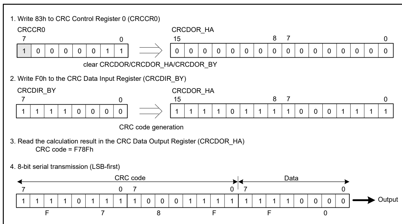
Figure 40.2 LSB-first data transmission
