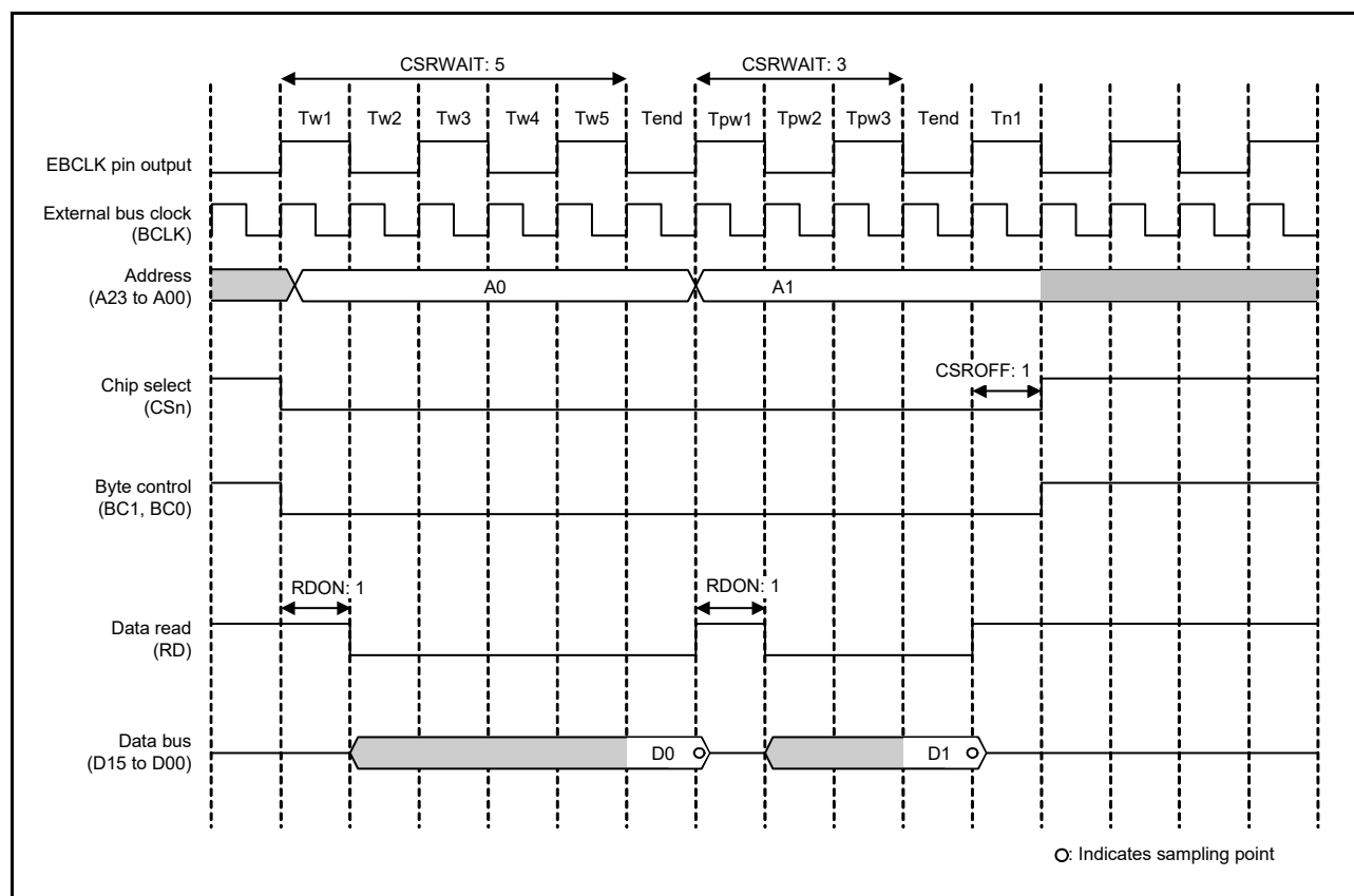
Figure 15.25 Example page read access operation when BCLK/2 is selected in the EBCLK Pin Output Select bit and two rounds of bus access are generated in response to a single transfer request ( n = 0 to 7)
