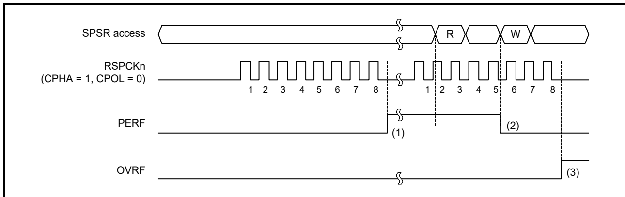
Figure 38.31 Operation example of the PERF flag
