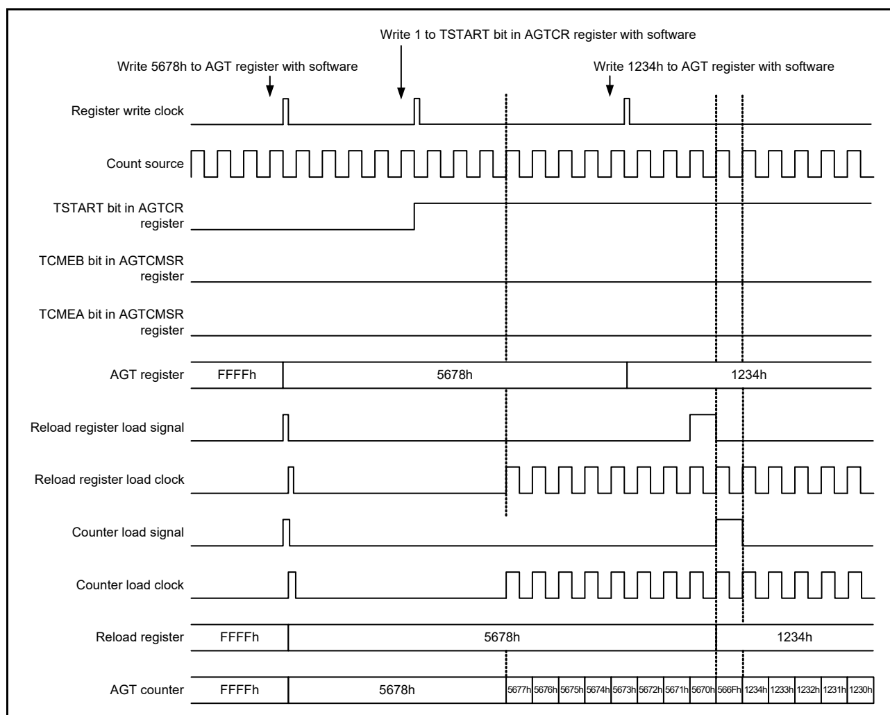
Figure 25.2 Timing of rewrite operation with TSTART bit value and TCMEA and TCMEB bit value when compare match register A and B are invalid
