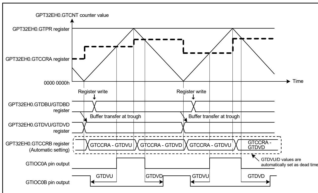
Figure 23.46 Example of automatic compare-match value setting function with dead time, with triangle-wave PWM mode 2 or 3, GTDVU and GTDDVD set to buffer operation, and active-high
