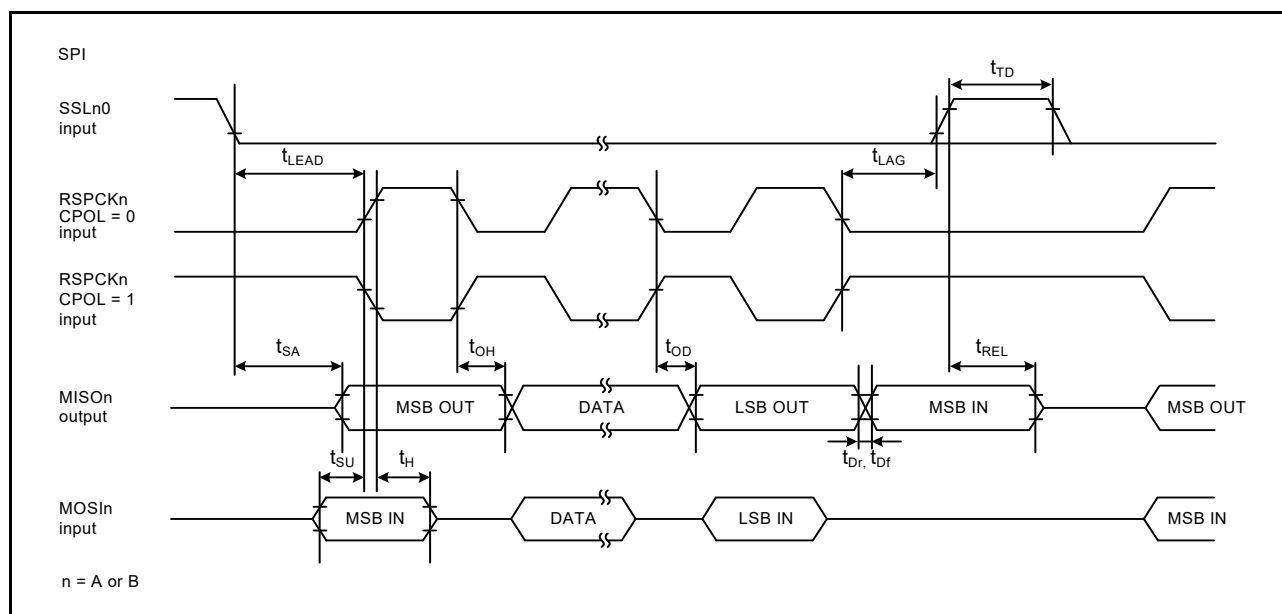
Figure 60.56 SPI timing for slave when CPHA = 0
