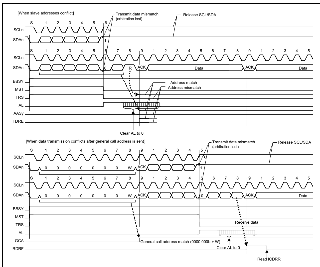
Figure 36.41 Examples of master arbitration-lost detection when MALE = 1
