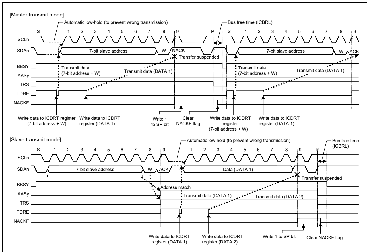
Figure 36.39 Suspension of data transfer when NACK is received, when NACK = 1
