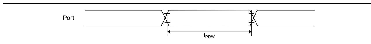
Figure 60.34 I/O ports input timing
