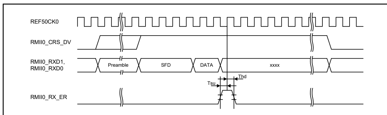
Figure 60.70 RMII reception timing when an error occurs
