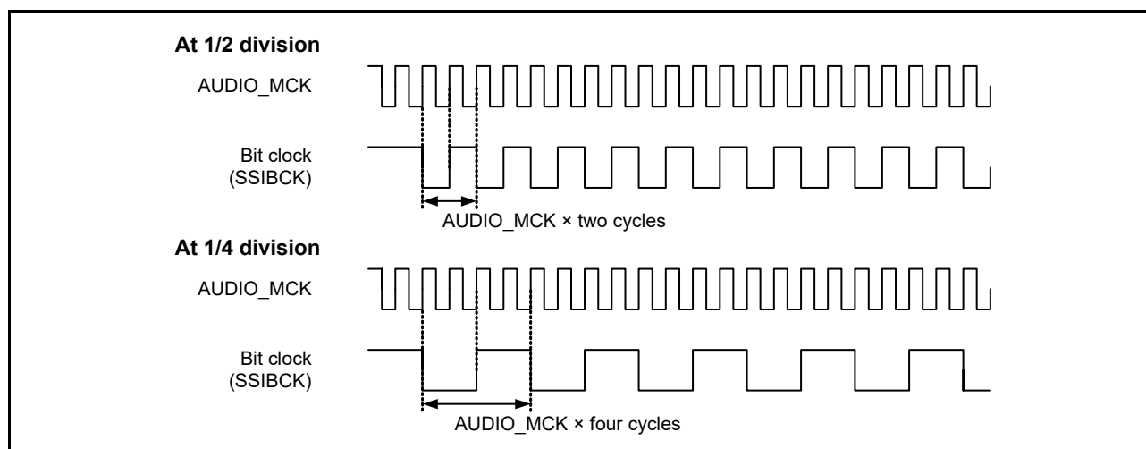
Figure 41.6 Sampling frequencies in master-mode communication
