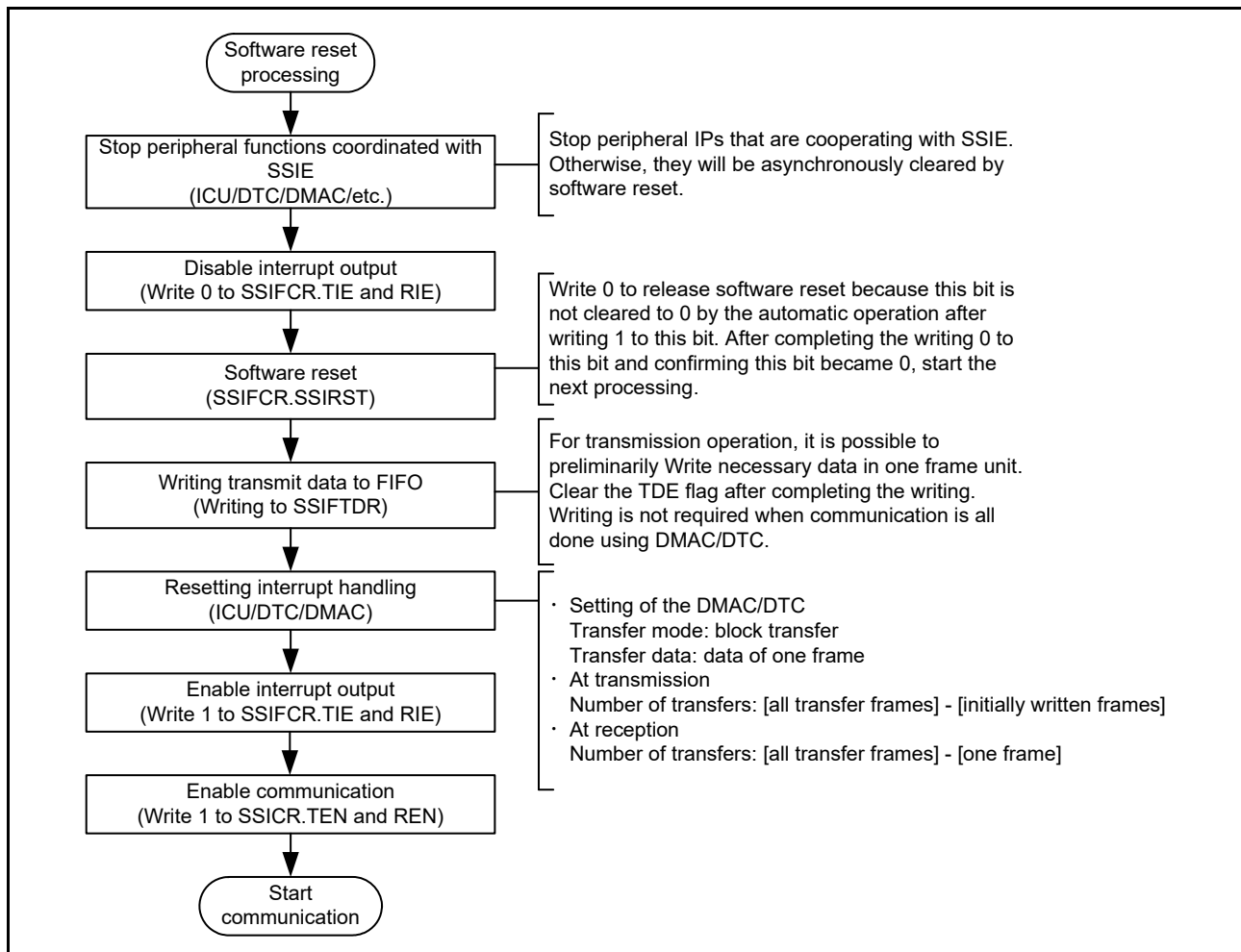
Figure 41.62 Software reset procedure (CPU operation procedure)
