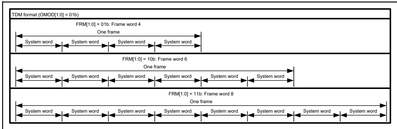
Figure 41.13 Frame word number
