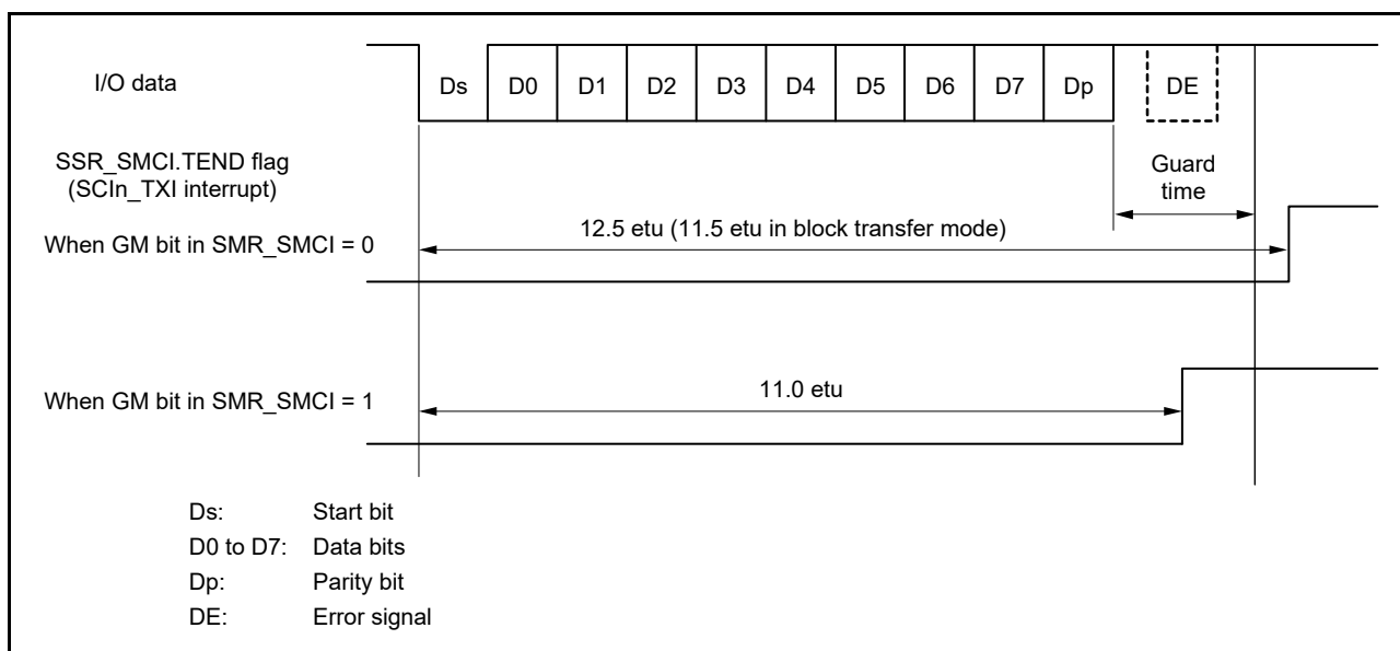
Figure 34.53 SSR.TEND flag generation timing during transmission
