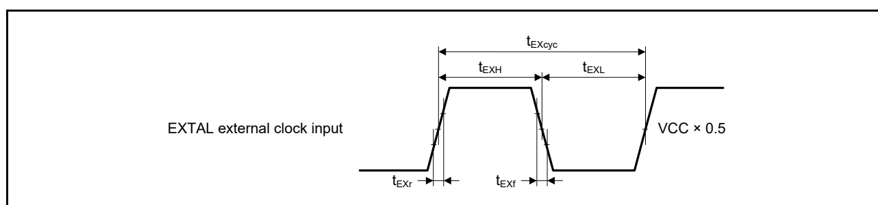
Figure 60.8 EXTERNAL external clock input timing
