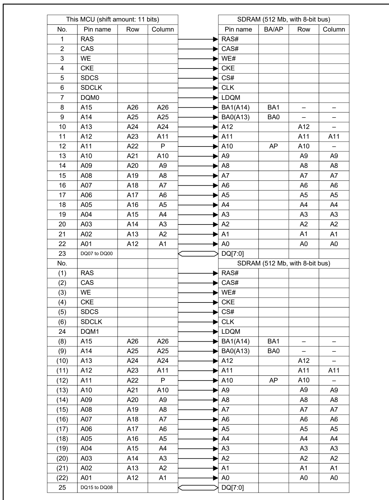
Figure 15.70 SDRAM connection example with 512-Mb × 2 and 8-bit bus
