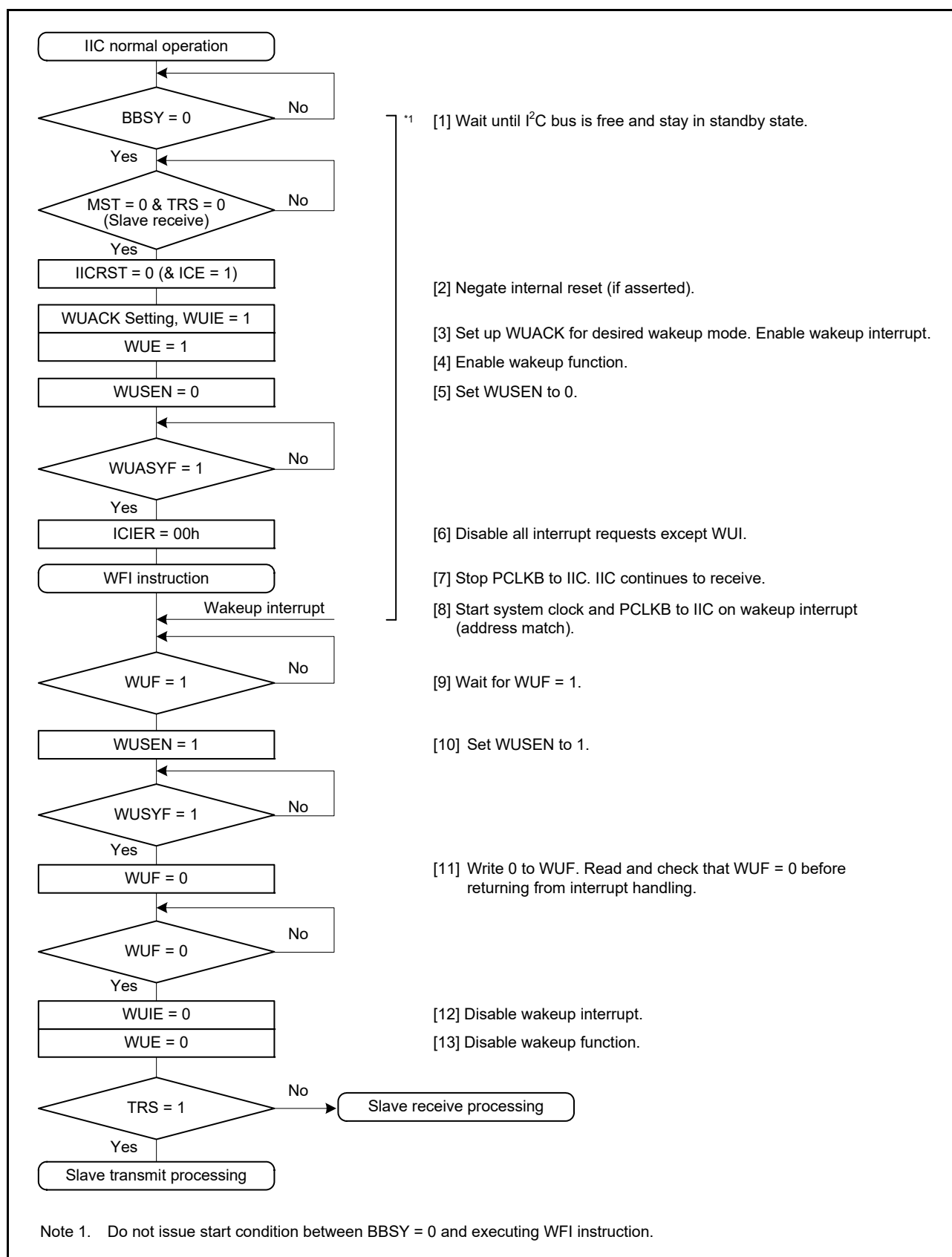
Figure 36.33 Example operation of normal wakeup mode 2 when wakeup is triggered by a wakeup interrupt on match of the slave address
