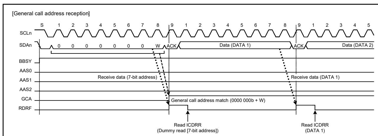
Figure 36.27 Timing of GCA flag setting during reception of general call address
