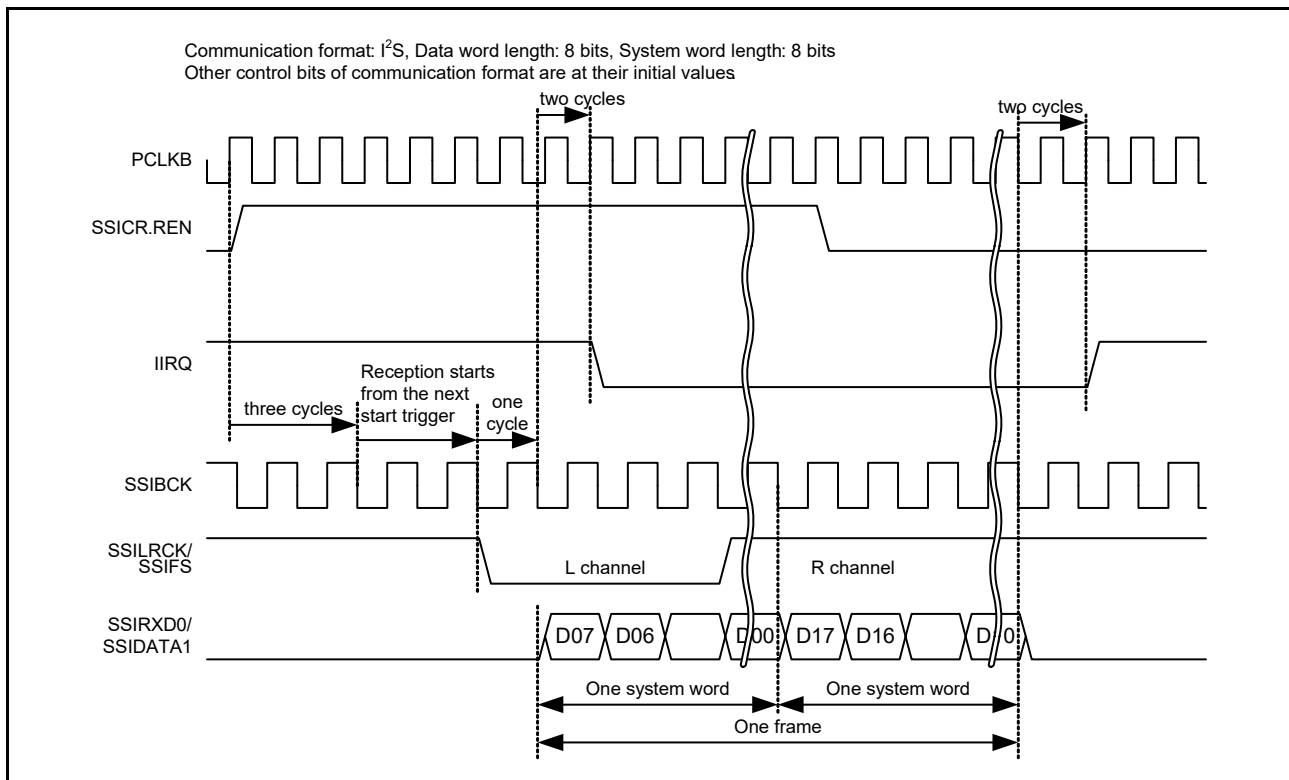
Figure 41.15 IIRQ setting timing (reception)
