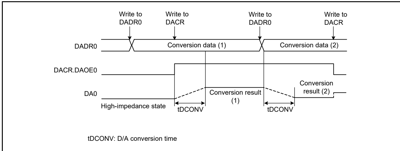
Figure 48.2 Example of DAC12 operation
