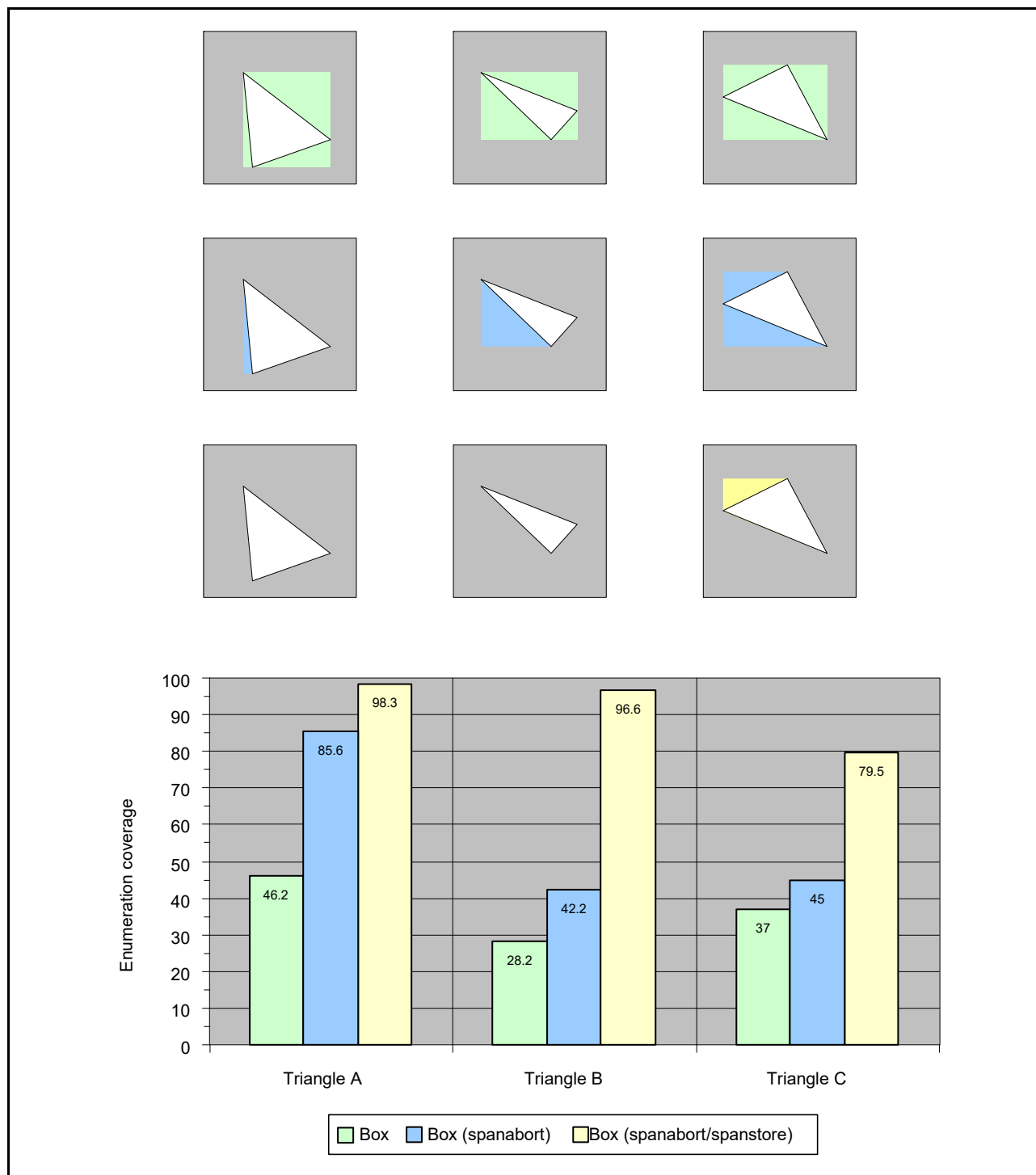
Figure 56.19 Efficiency of spanstore and spanabort optimizations with enumeration coverage equal to {pixels of primitive/pixels of bounding box}
