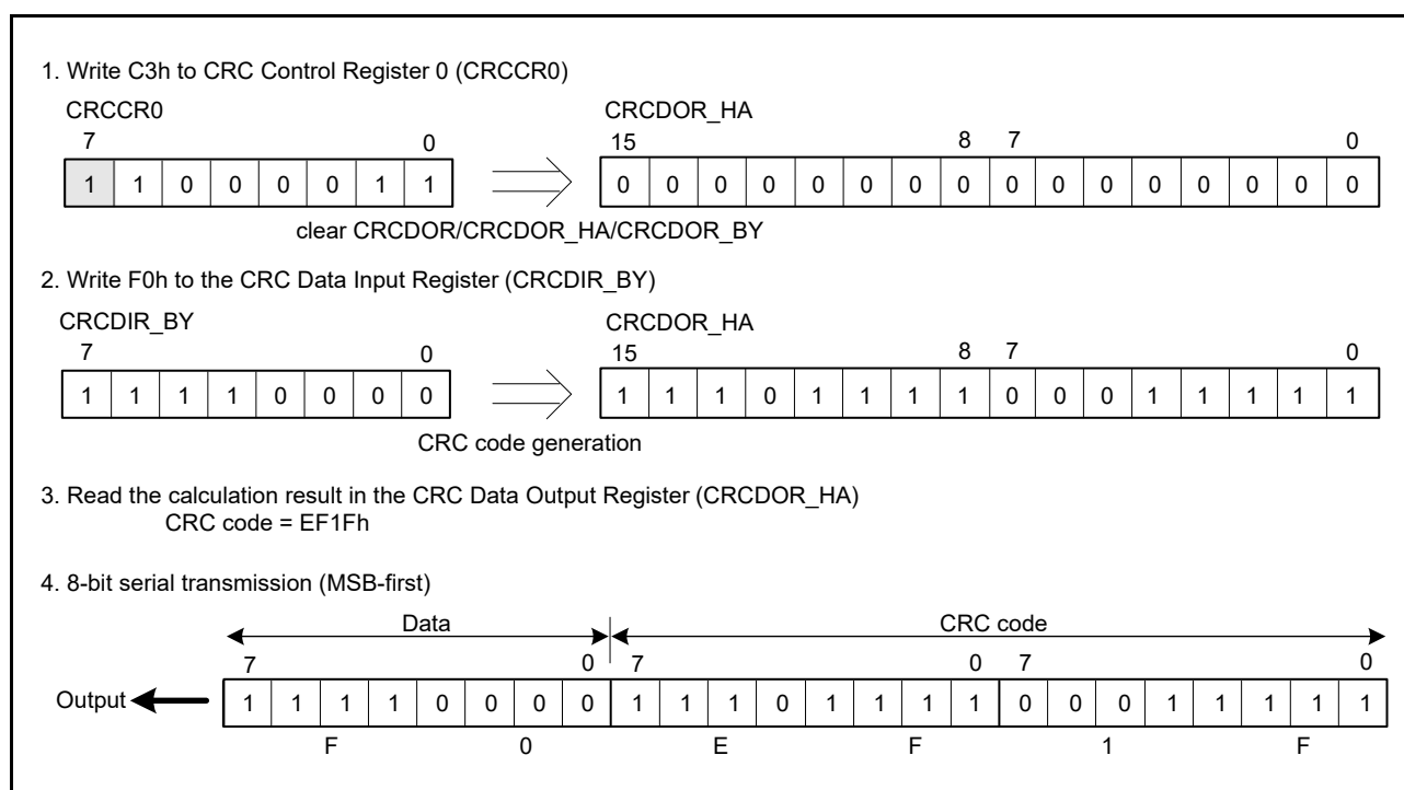
Figure 40.3 MSB-first data transmission
