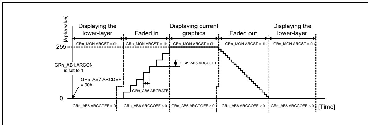
Figure 58.11 Changes in alpha value
