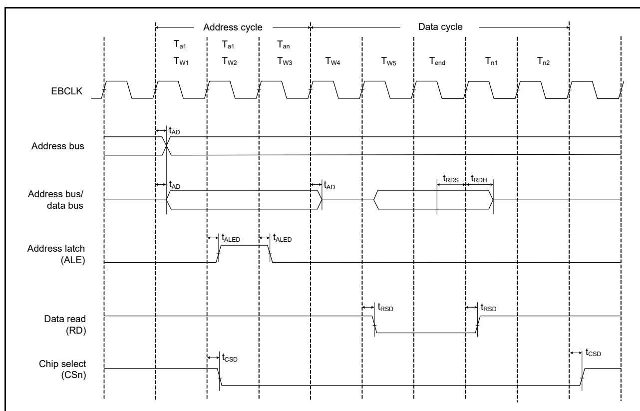
Figure 60.20 Address/data multiplexed bus read access timing
