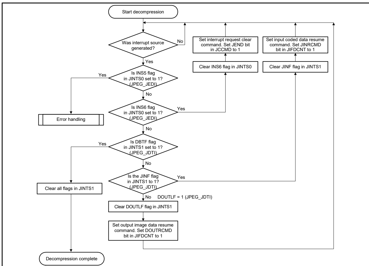
Figure 57.9 Decompression process flow
