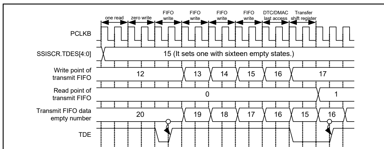
Figure 41.29 Timing diagram for setting and clearing TDE
