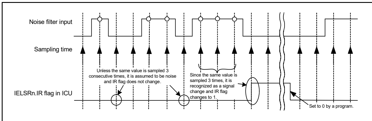
Figure 50.4 Noise filter and interrupt operation example
