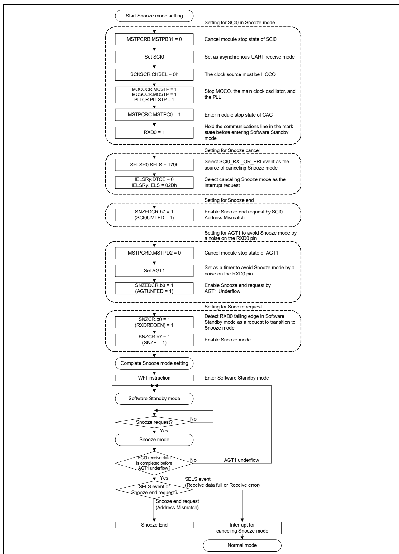
Figure 11.9 Setting example of using SCI0 in Snooze mode entry
