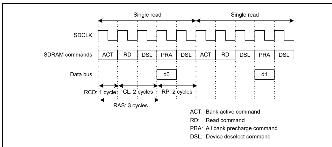
Figure 15.54 Example timing for single read (1)
