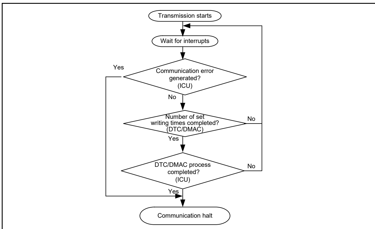
Figure 41.54 Transmission procedure
