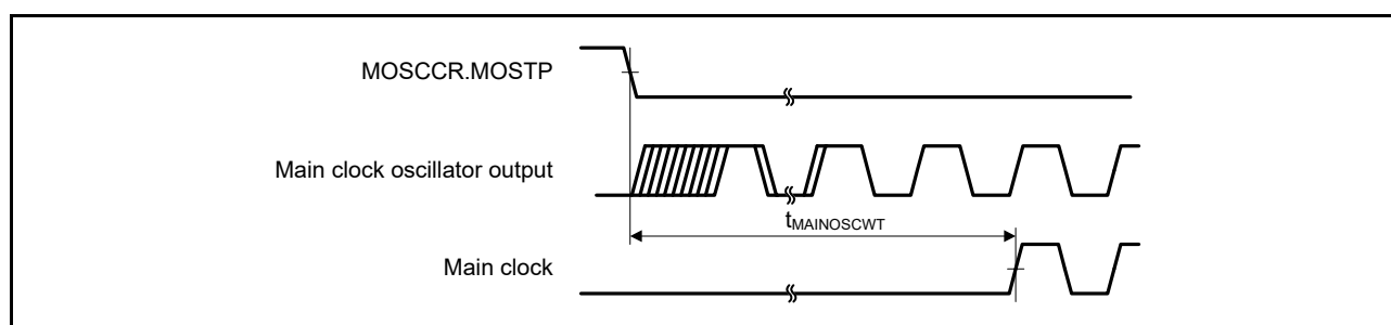
Figure 60.9 Main clock oscillation start timing
