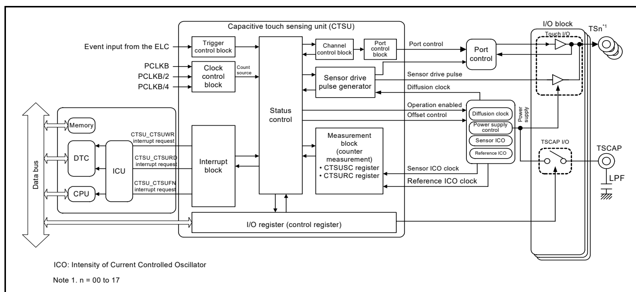
Figure 51.3 CTSU block diagram
