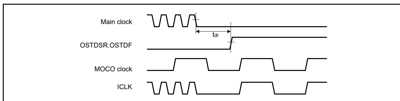
Figure 60.96 Oscillation stop detection timing
