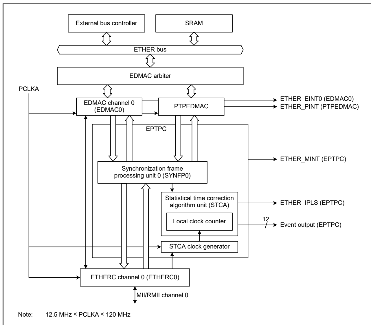
Figure 30.1 EPTPC configuration
