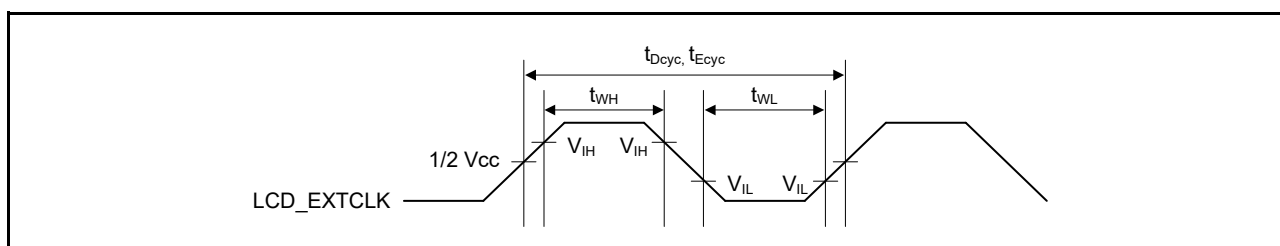
Figure 60.80 LCD_EXTCLK clock input timing
