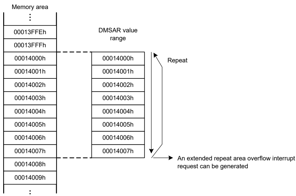
Figure 17.5 Example of extended repeat area operation
