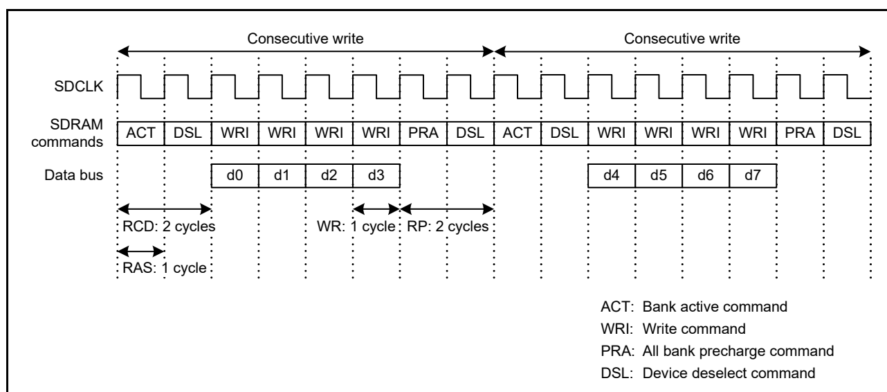
Figure 15.68 Example timing for consecutive write (2)
