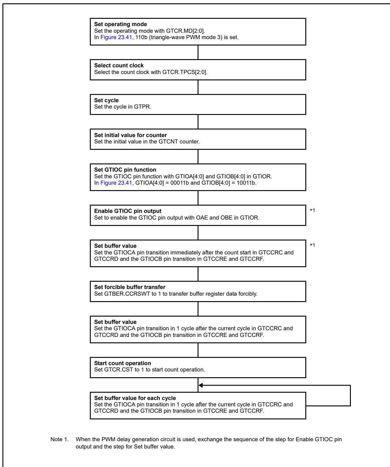
Figure 23.42 Example setting for triangle-wave PWM mode 3
