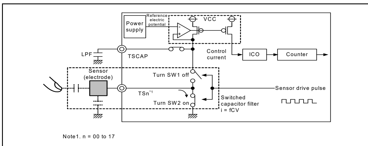
Figure 51.6 Discharging operation
