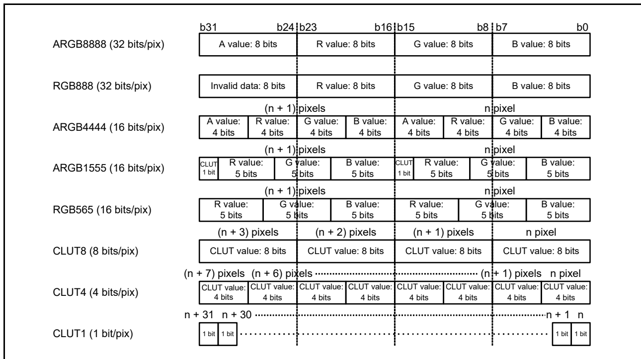
Figure 58.4 Frame data format
