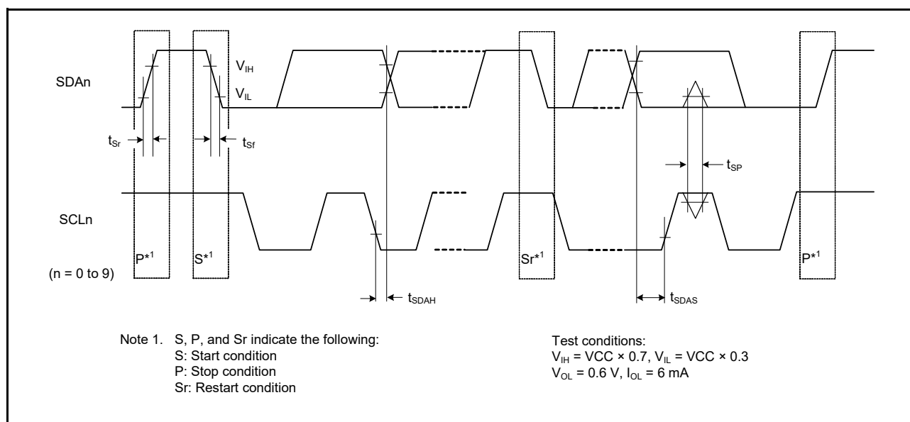
Figure 60.50 SCI simple IIC mode timing
