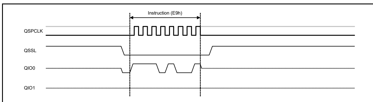
Figure 39.27 Exit 4-Byte Mode bus cycle
