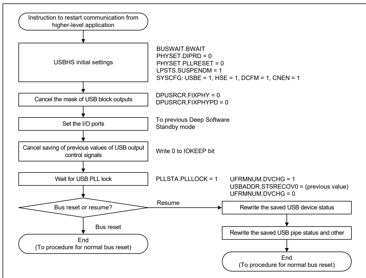
Figure 33.24 USBHS setup flow for canceling Deep Software Standby mode as a host controller (2)
