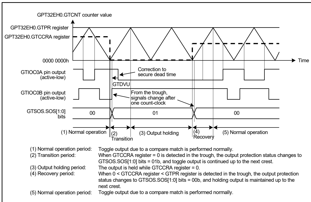
Figure 23.98 Example of output protection operation when GTCCR.A is set to 0 during buffer transfer at troughs, with 0 < \text{GTCCR.A} < \text{GTPR} restored during buffer transfer at troughs, and active-low
