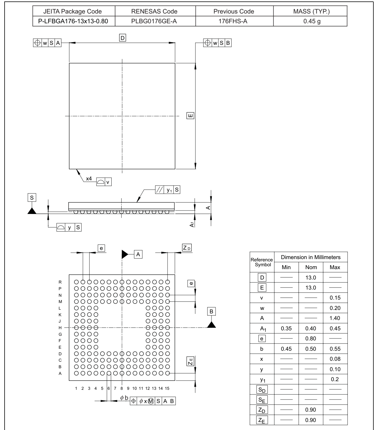
Figure 2.1 176-pin BGA
