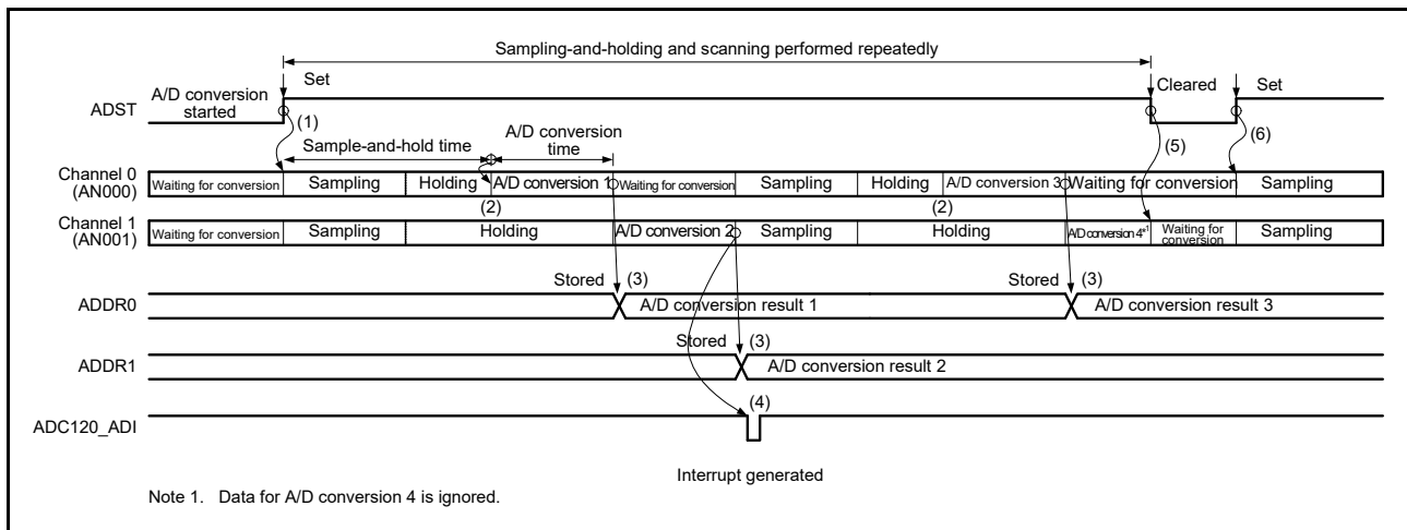
Figure 47.17 Example operation in continuous scan mode when channel-dedicated sample-and-hold circuits are used and AN000 and AN001 are selected
