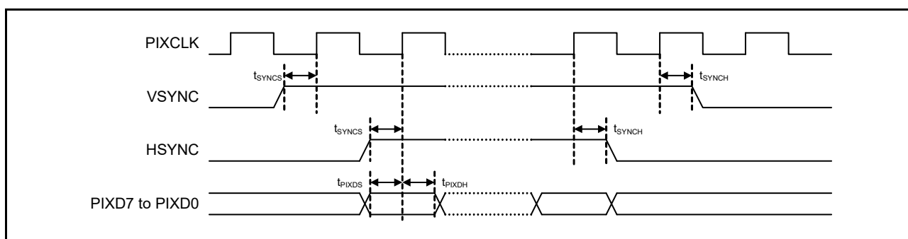
Figure 60.79 PDC AC timing
