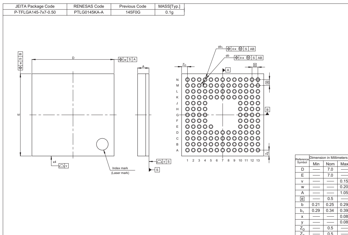
Figure 2.3 145-pin LGA
