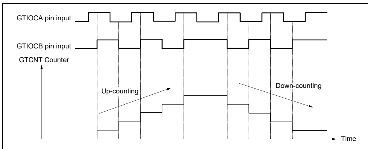
Figure 23.78 Example of phase counting mode 4
