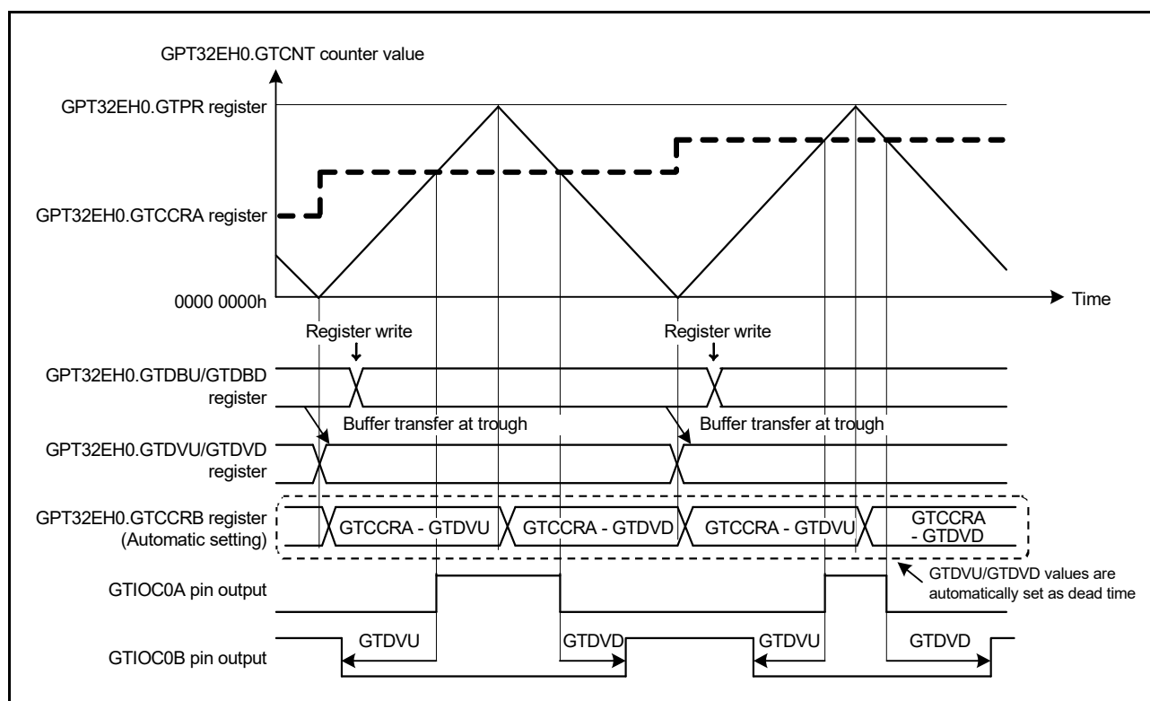
Figure 23.45 Example of automatic compare-match value setting function with dead time with triangle-wave PWM mode 1, GTDVU and GTDDVD set to buffer operation, active-high
