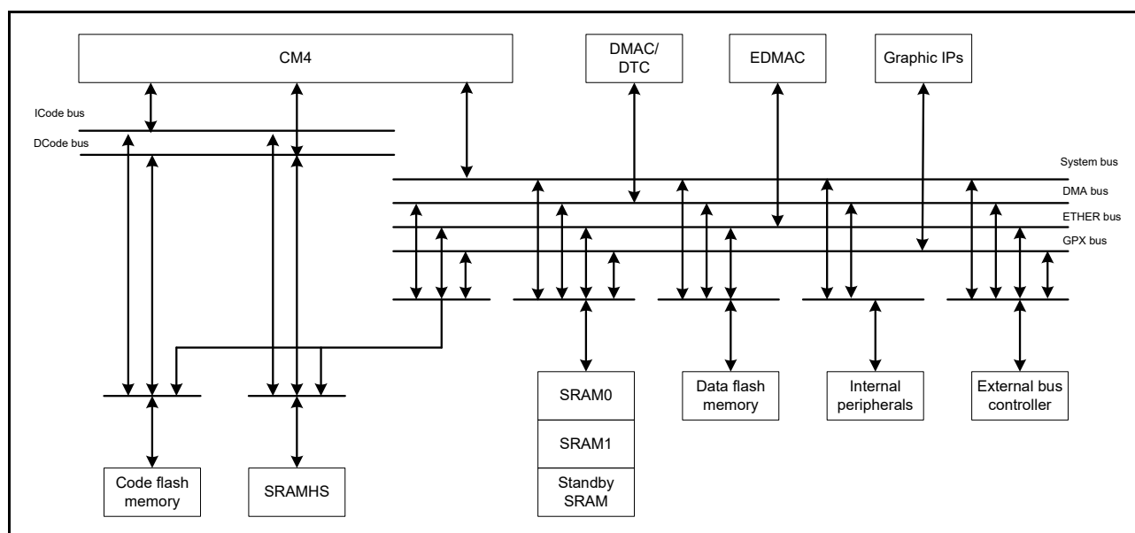
Figure 15.1 Bus configuration
