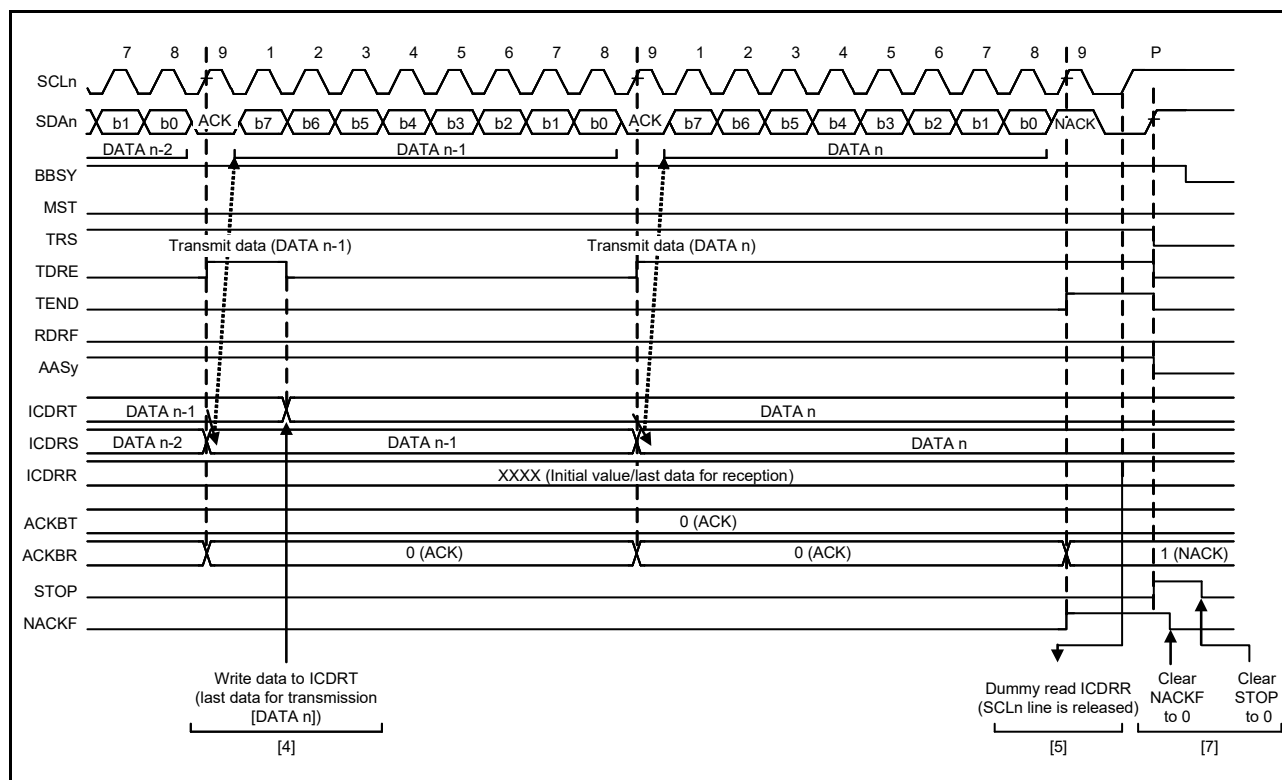
Figure 36.17 Slave transmit operation timing (2)
