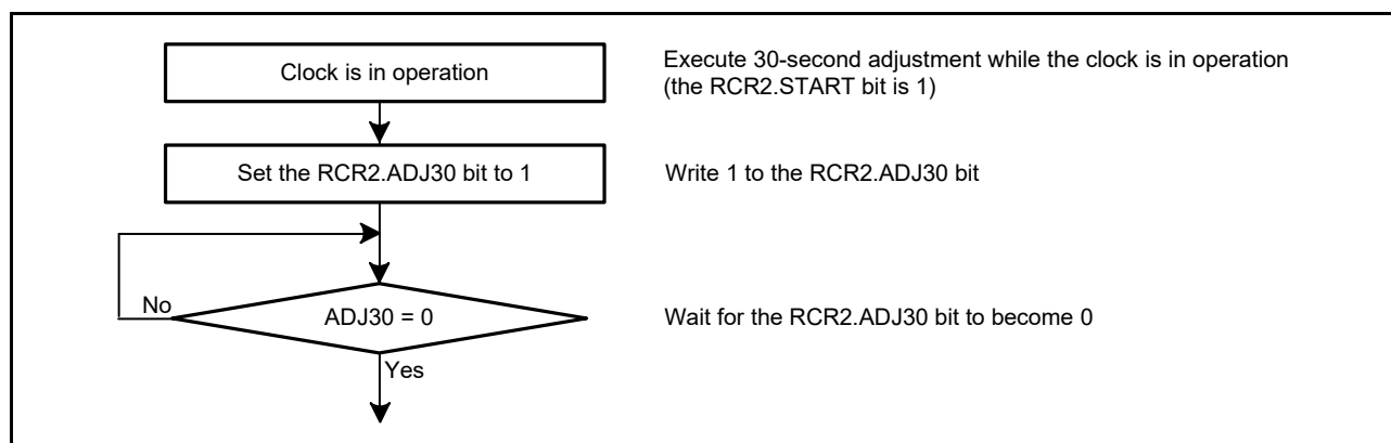
Figure 26.5 30-second adjustment
