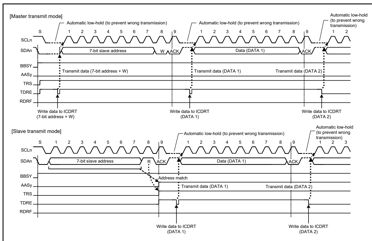
Figure 36.38 Automatic low-hold operation in transmit mode
