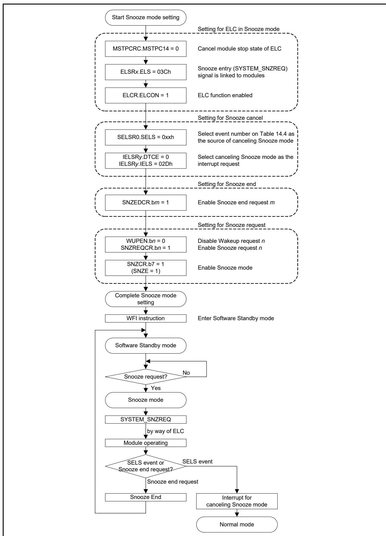
Figure 11.8 Setting example of using ELC in Snooze mode
