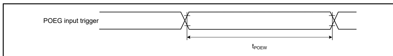
Figure 60.35 POEG input trigger timing
