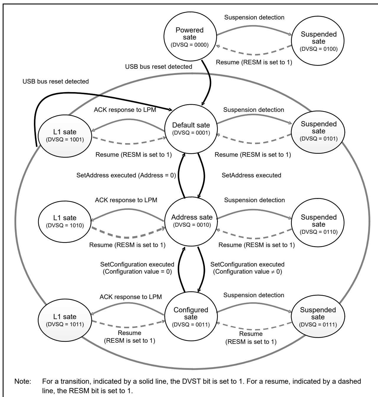
Figure 33.8 Device state transitions
