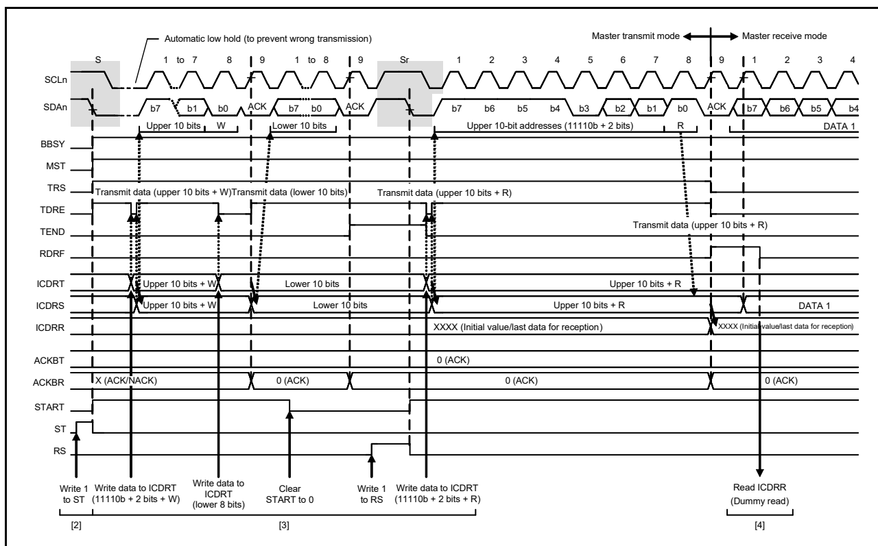
Figure 36.13 Master receive operation timing (2) with 10-bit address format, when RDRFS = 0
