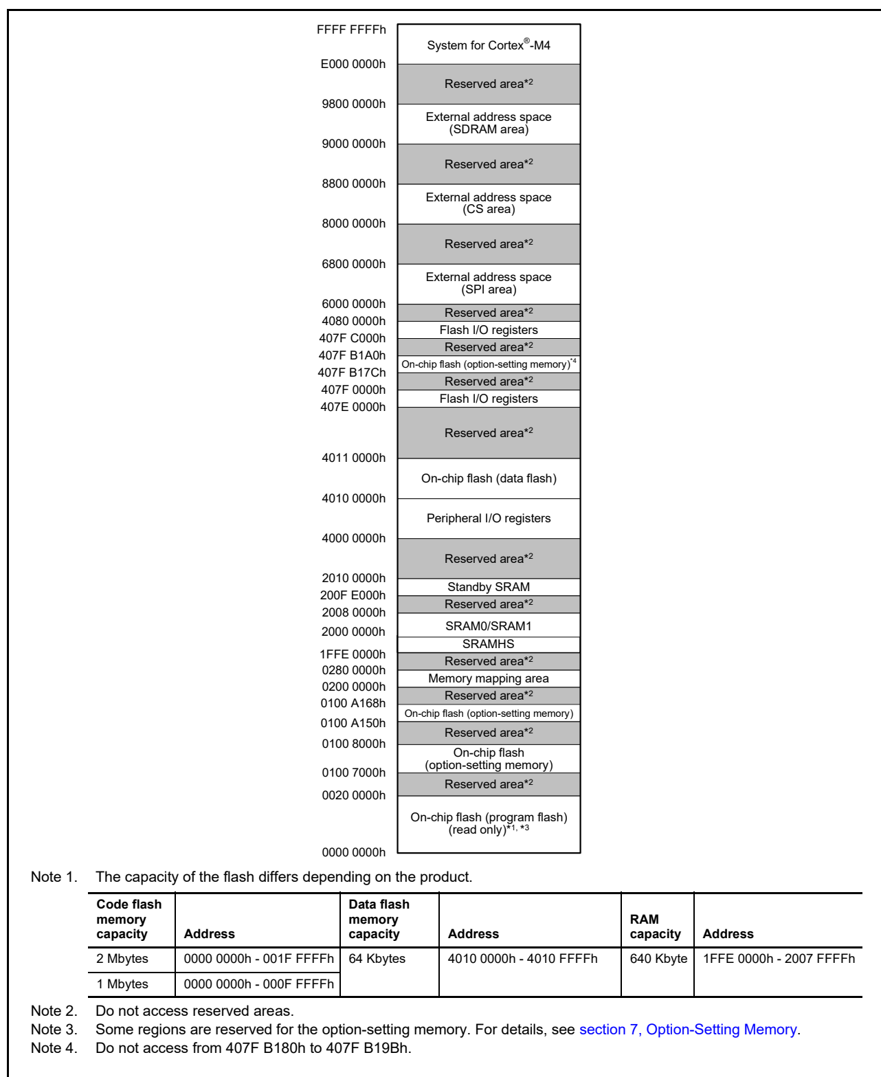
Figure 4.1 Memory map
