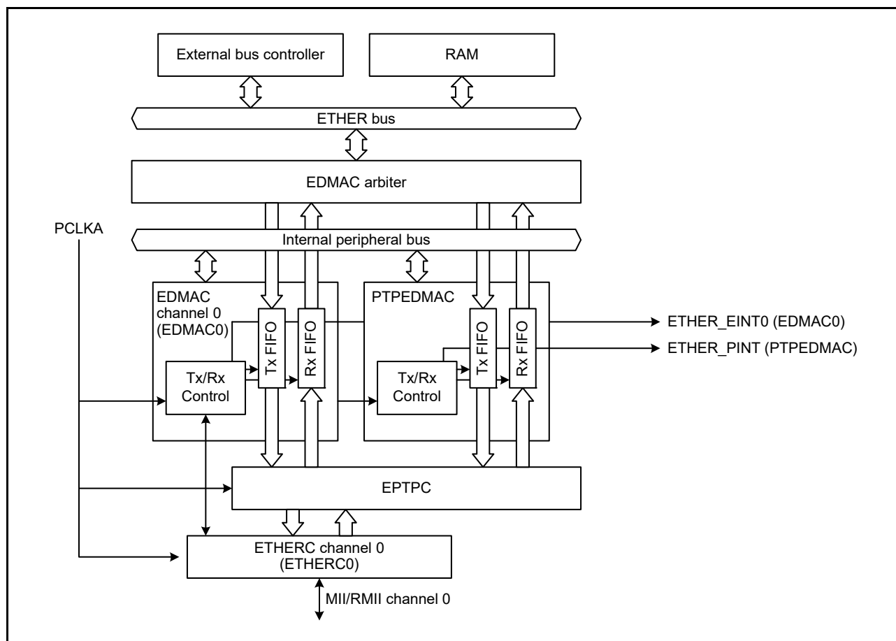
Figure 31.1 EDMAC configuration
