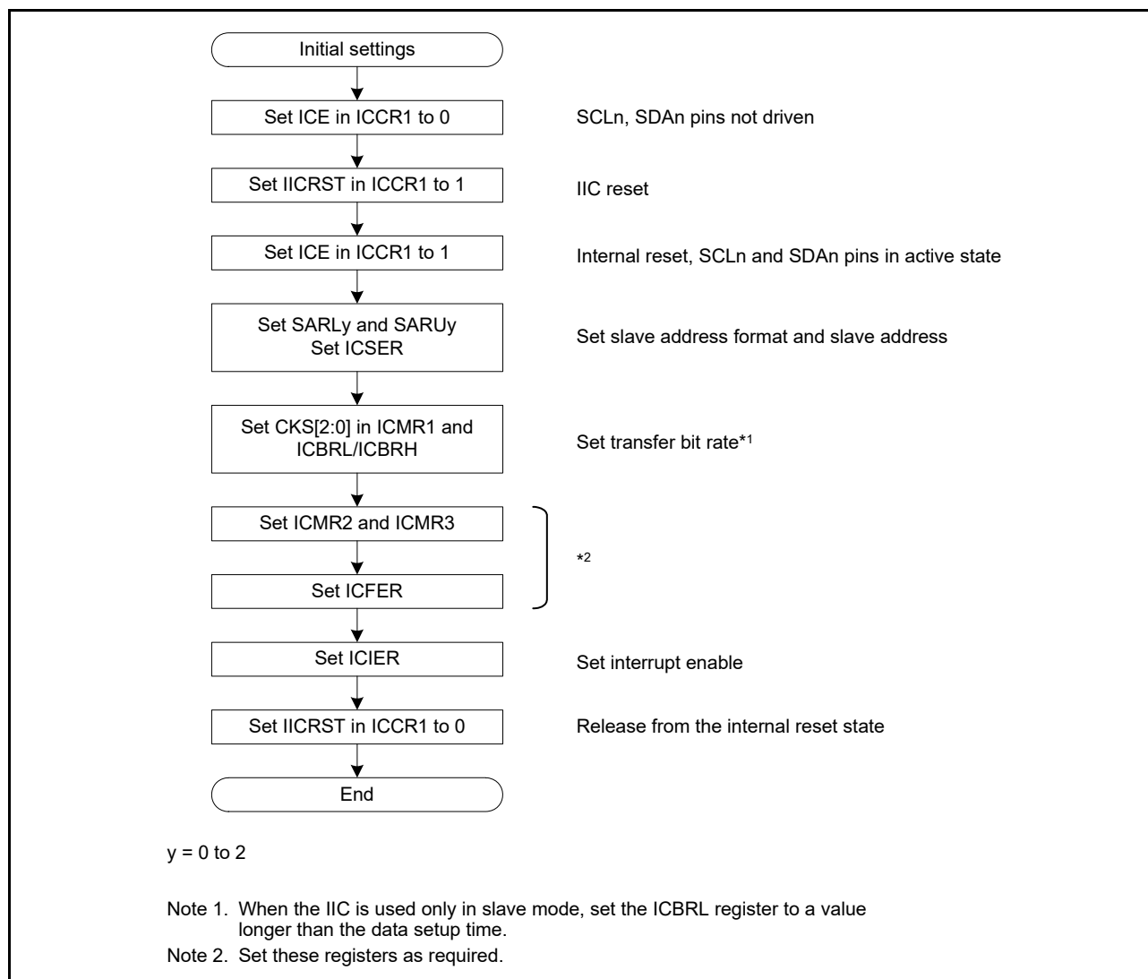
Figure 36.5 Example IIC initialization flow
