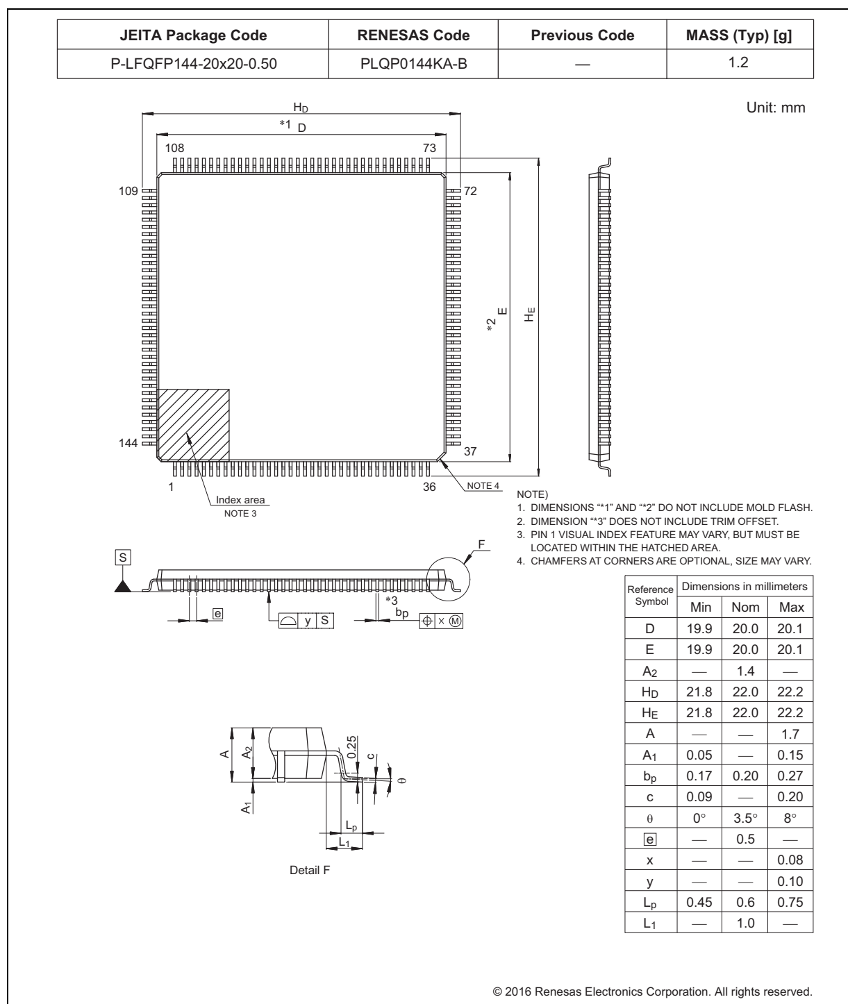
Figure 2.4 144-pin LQFP
