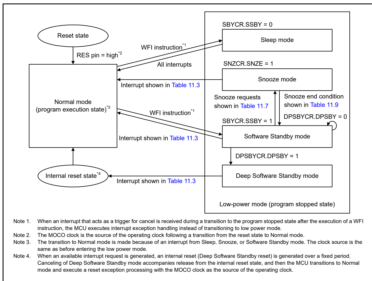
Figure 11.1 Mode transitions
