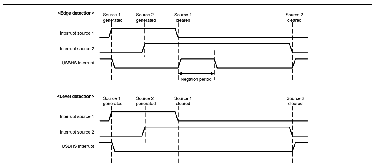
Figure 33.3 USBHS interrupt operation
