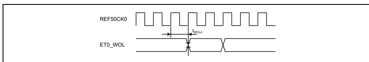
Figure 60.71 WOL output timing for RMII
