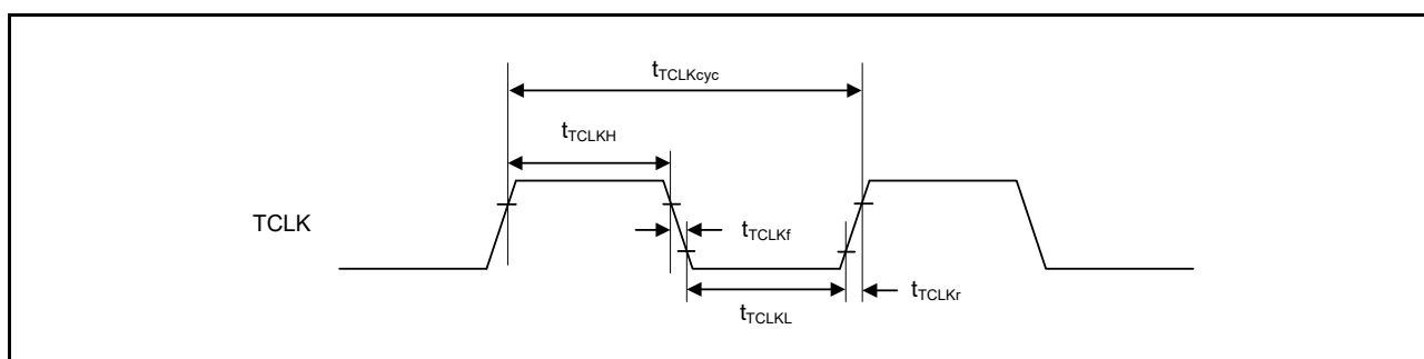
Figure 60.110 ETM TCLK timing
