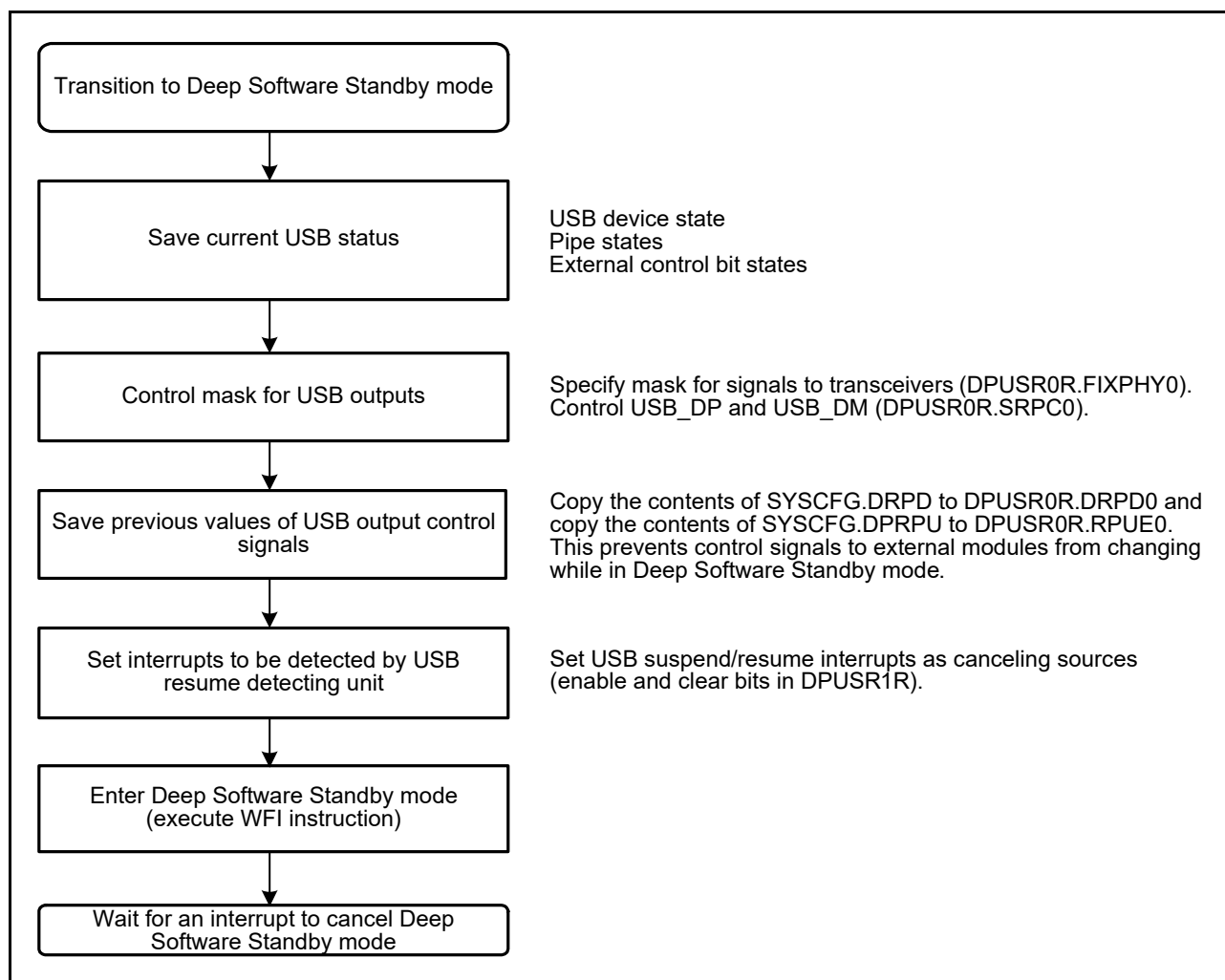
Figure 32.7 USBFS setup flow for transition to Deep Software Standby mode as host or device controller
