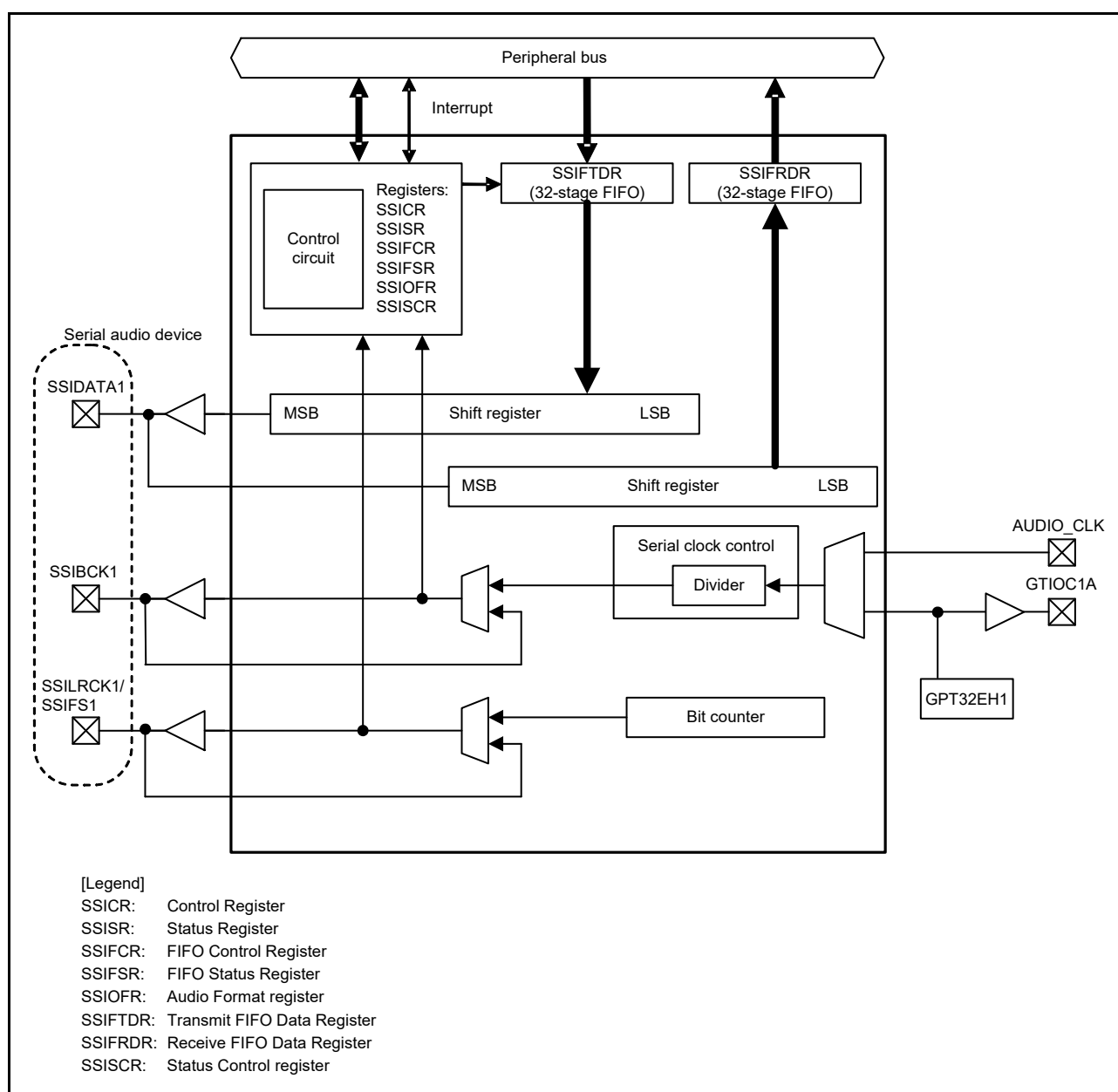
Figure 41.3 SSIE block diagram (SSIE1)
