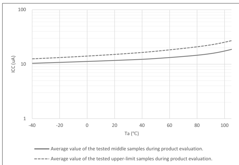
Figure 60.4 Temperature dependency in Deep Software Standby mode, power not supplied to SRAM or USB resume detecting unit, power-on reset circuit low-power function disabled (reference data)
