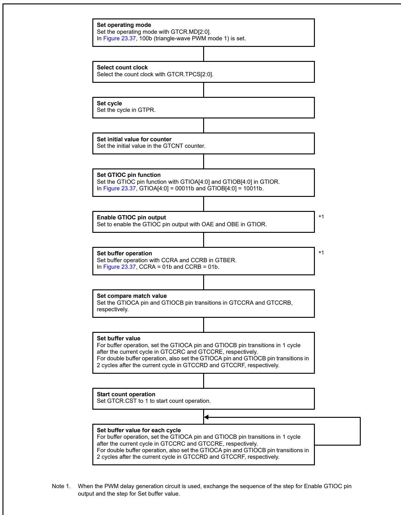
Figure 23.38 Example setting for triangle-wave PWM mode 1
