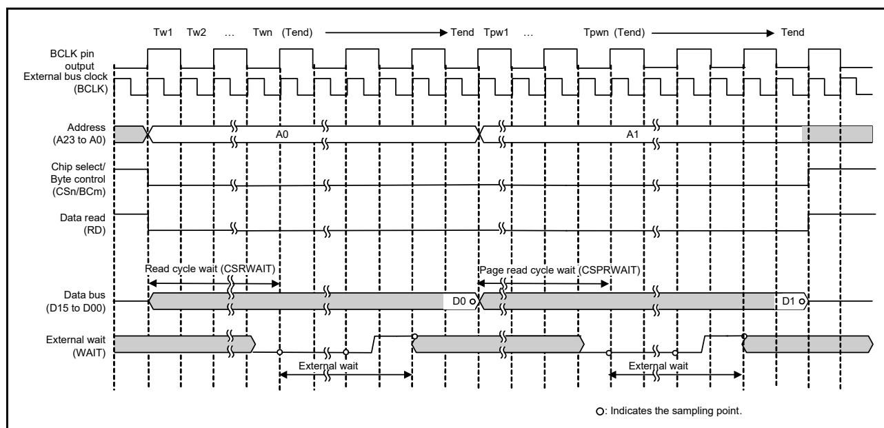
Figure 15.31 Example external wait timing for page read access to 16-bit bus space (when 1/2 BCLK is Selected with the BCLK Pin Output Select bit) ( n = 0 to 7 , m = 0, 1 )
