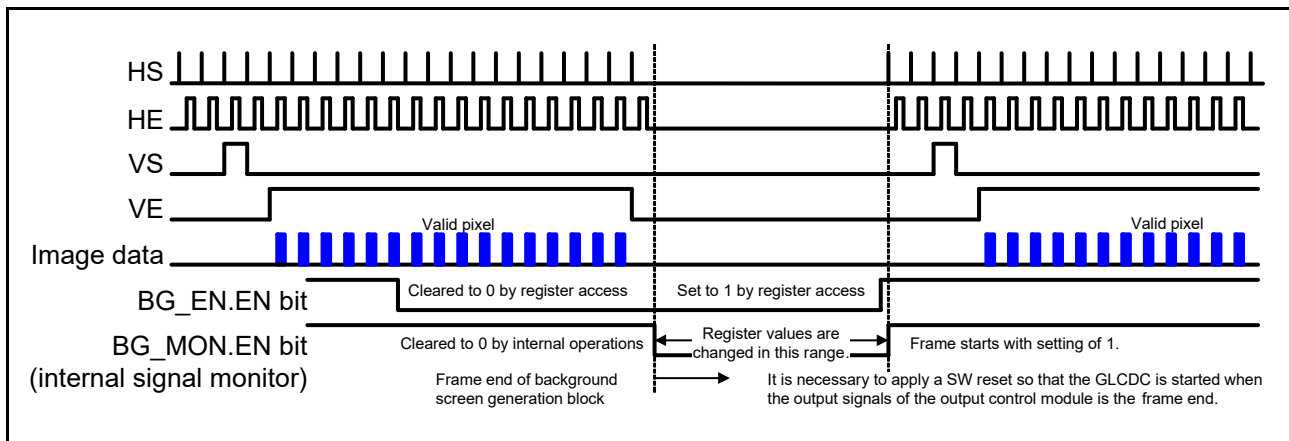
Figure 58.25 Stop and restart in normal operation
