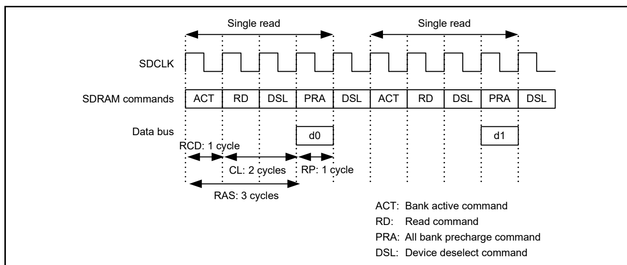
Figure 15.57 Example timing for single read (4)
