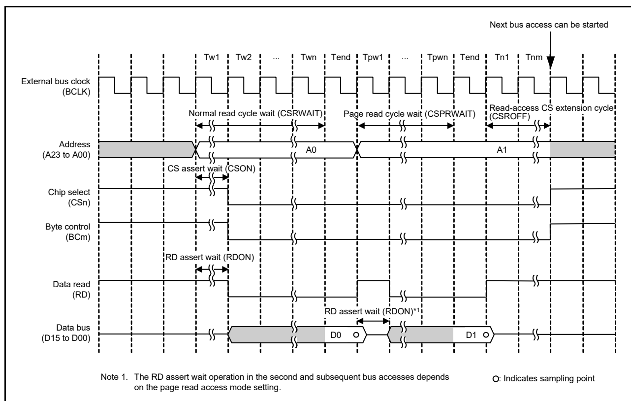
Figure 15.21 Page read access timing (n = 0 to 7, m = 0, 1)
