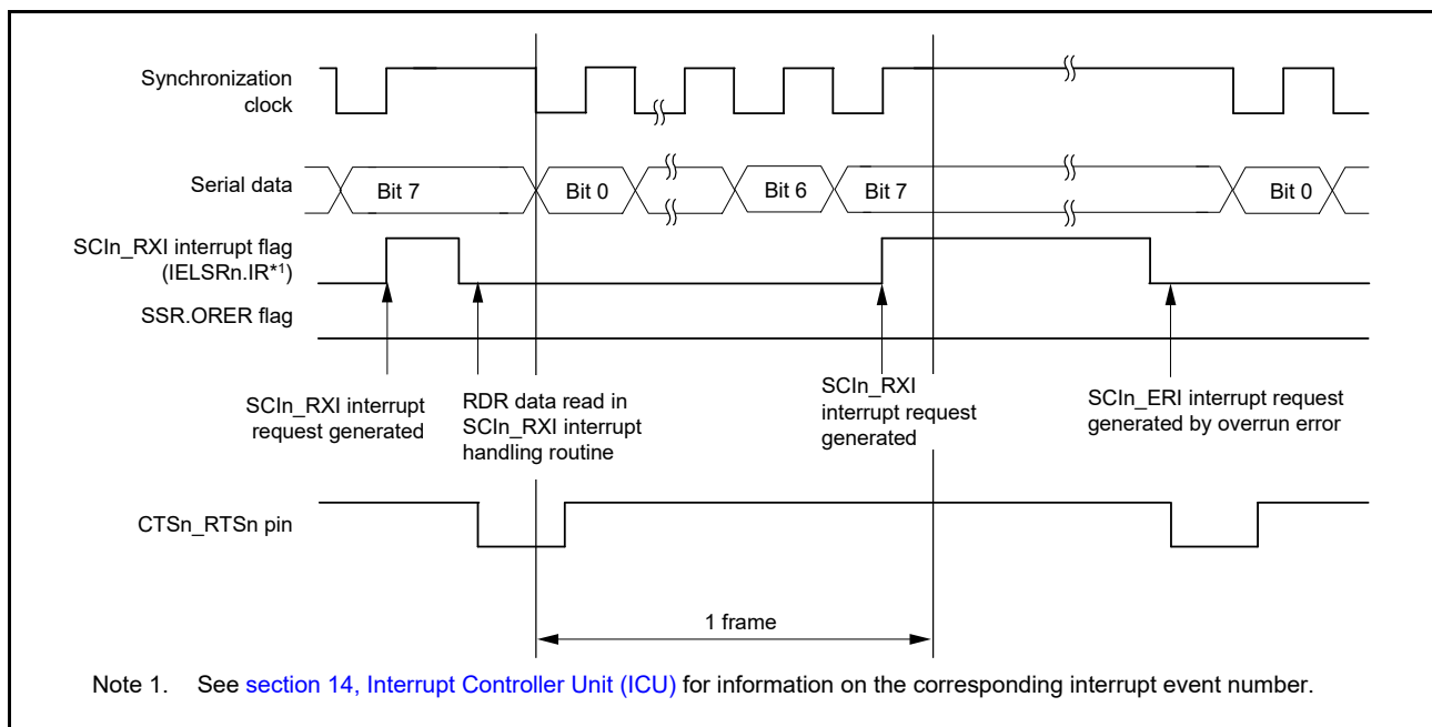
Figure 34.40 Example operation for serial reception in clock synchronous mode (2) when RTS function is used Data transfer cannot resume while the receive error flag is 1. Therefore, clear the ORER, FER, and PER bits in the SSR
