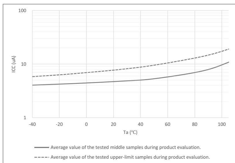
Figure 60.5 Temperature dependency in Deep Software Standby mode, power not supplied to SRAM or USB resume detecting unit, power-on reset circuit low-power function enabled (reference data)
