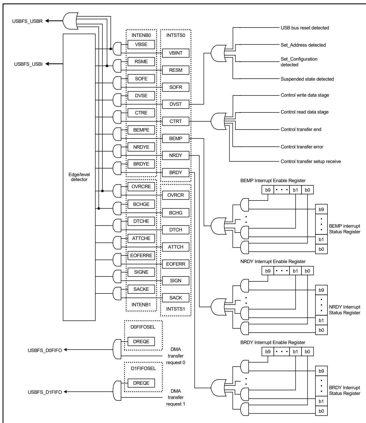
Figure 32.10 USBFS interrupt-related circuits
