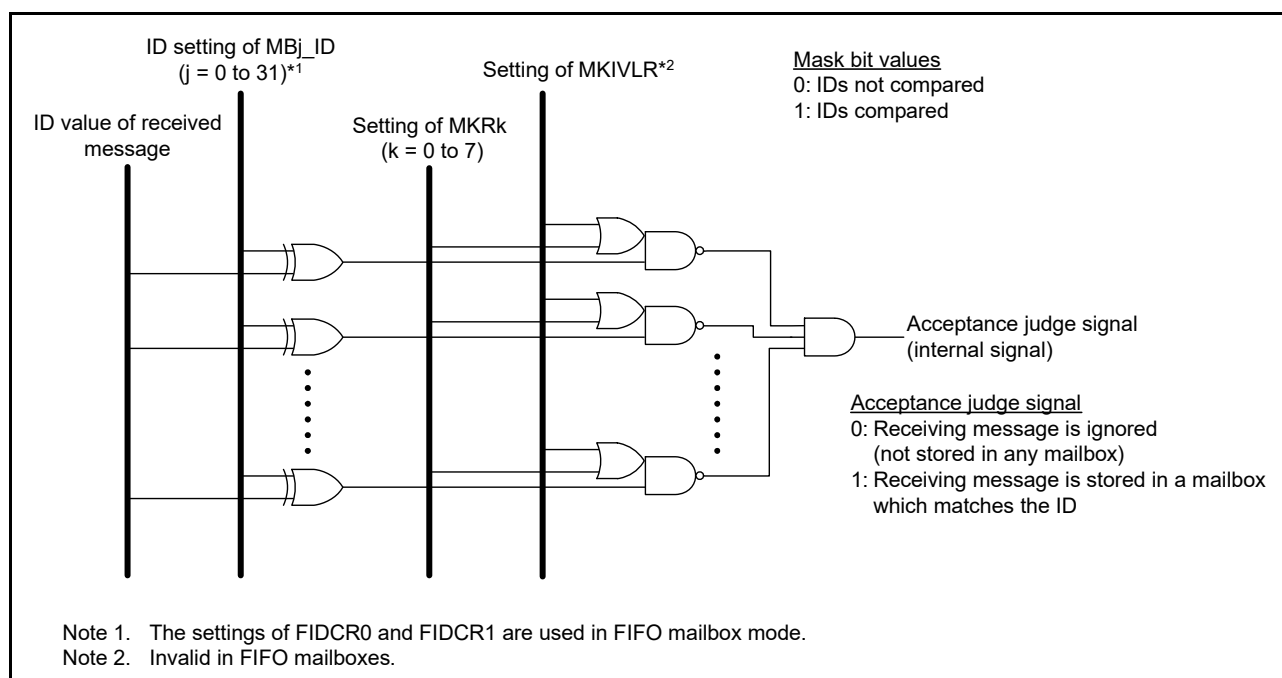
Figure 37.17 Acceptance filtering
