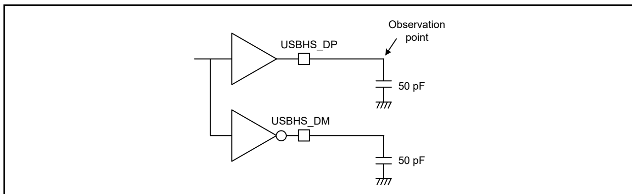
Figure 60.86 Test circuit in full-speed mode
