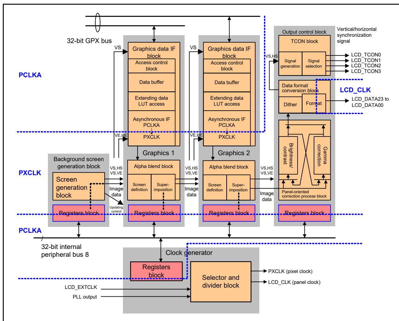
Figure 58.2 GLCDC configuration
