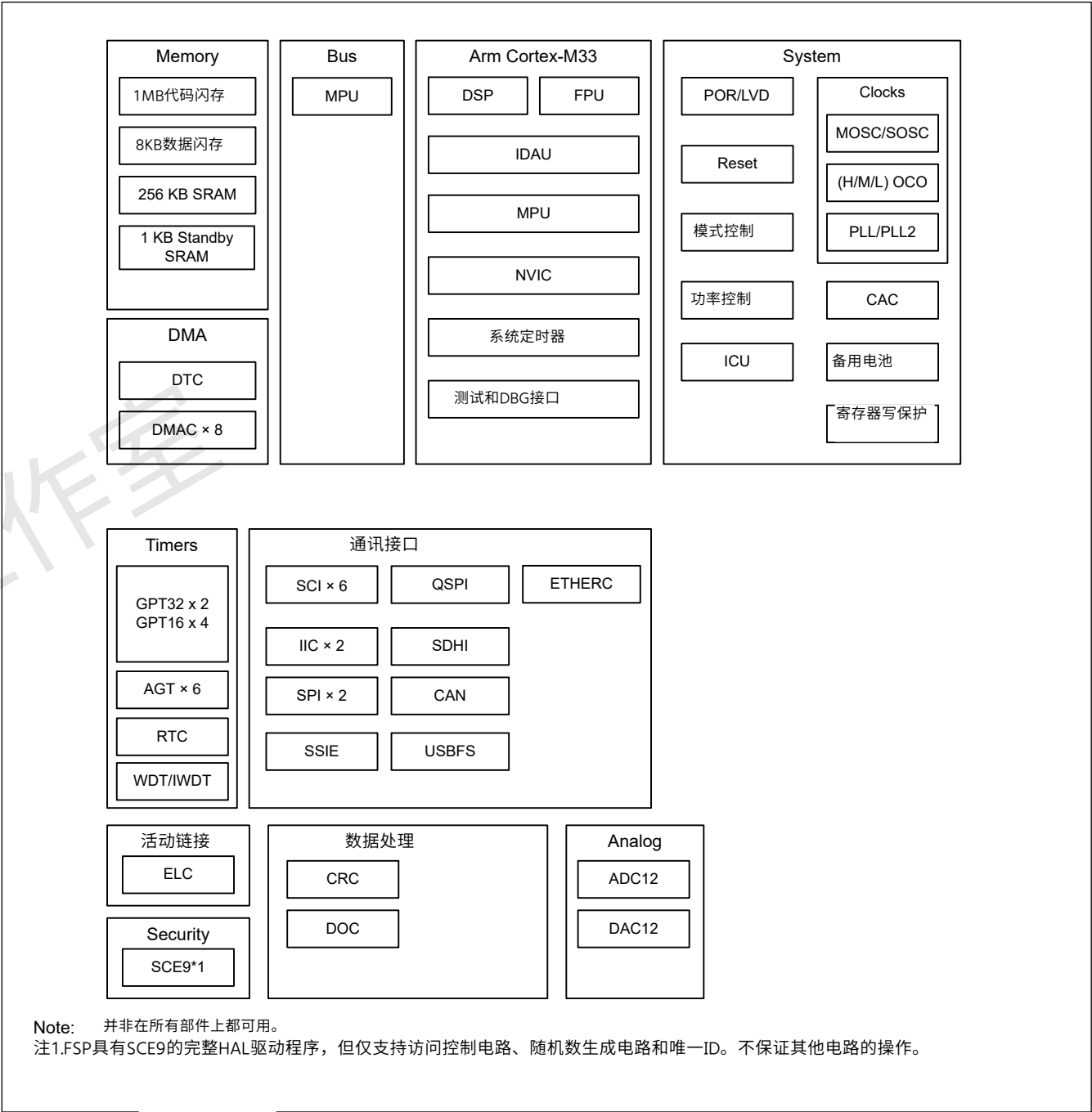
Figure 1.1 框图
