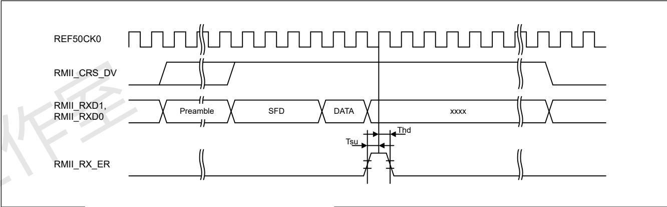
Figure 2.52 发生错误时的RMII接收时序
