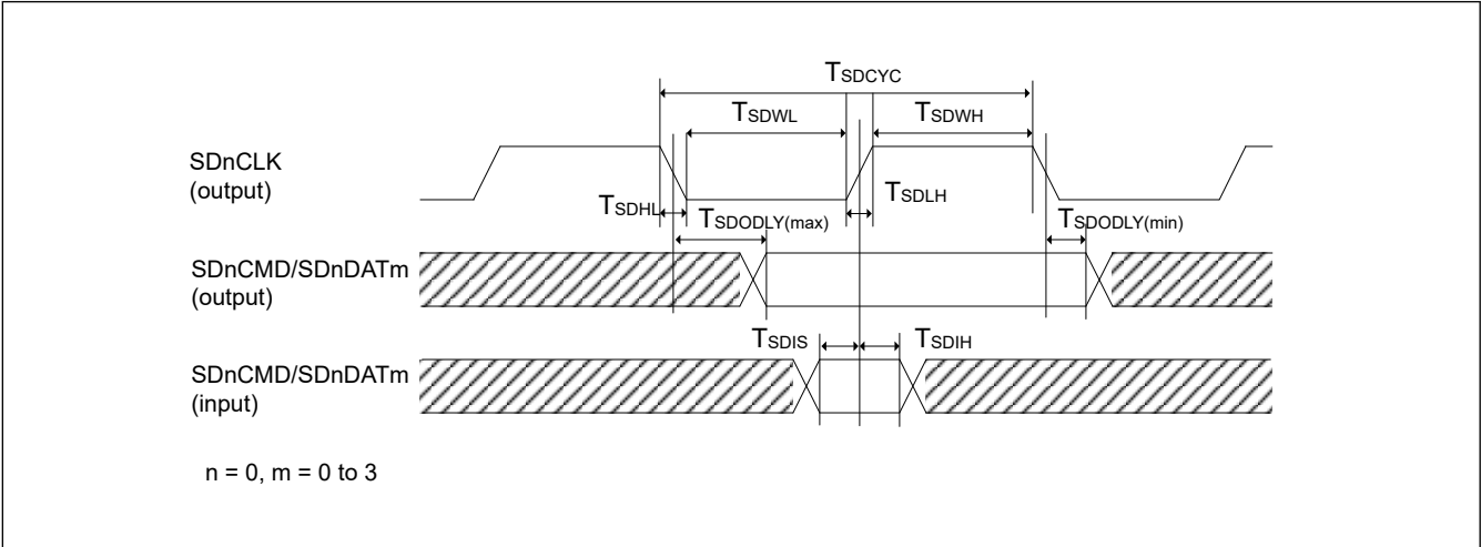
Figure 2.48 SDMMC主机接口信号时序
