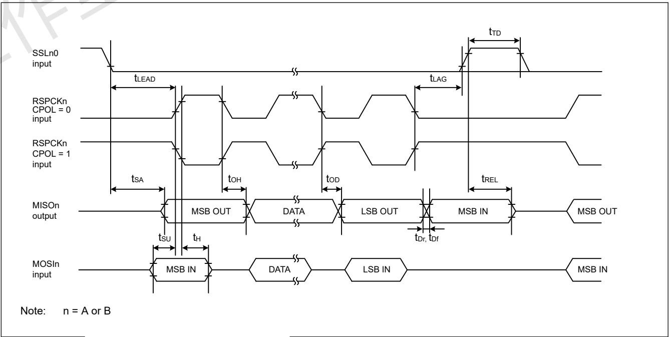
Figure 2.38 CPHA=0时从机的SPI时序
