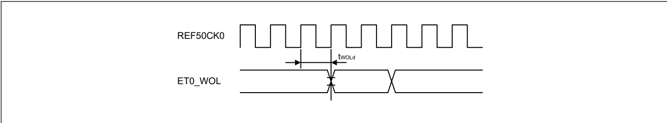
Figure 2.53 RMII的WOL输出时序
