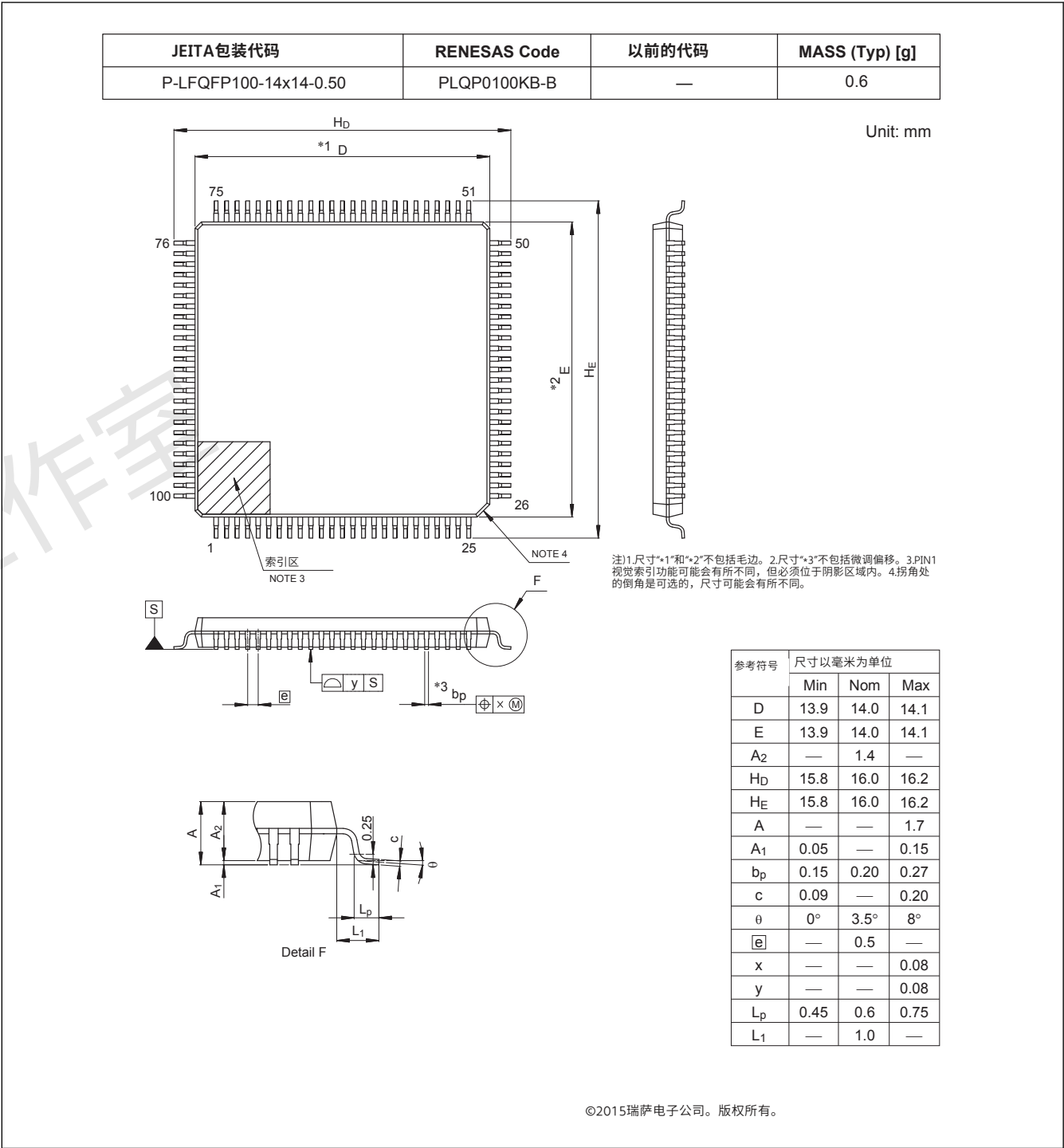
Figure 2.1 LQFP 100-pin
