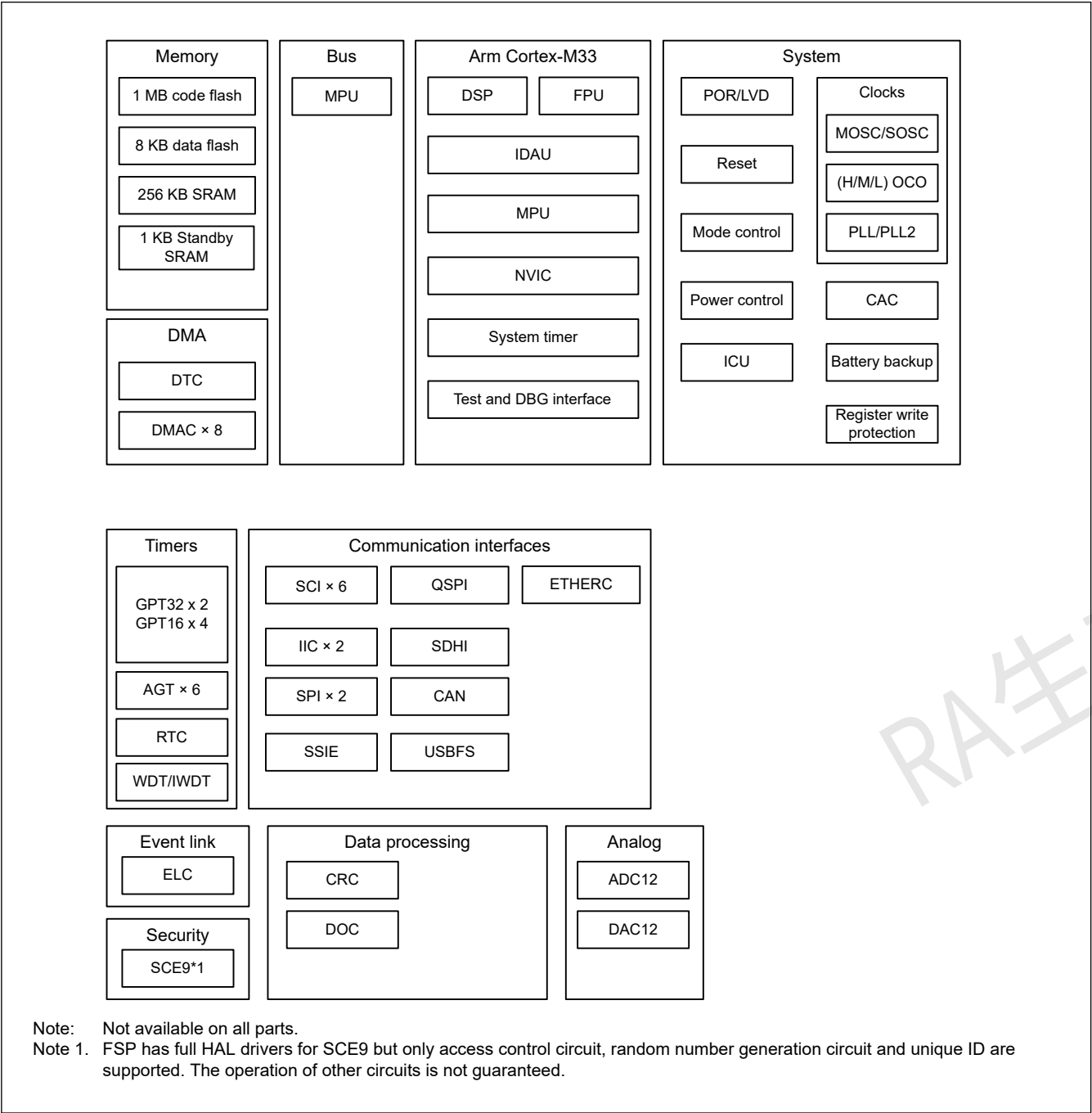
Figure 1.1 Block diagram
