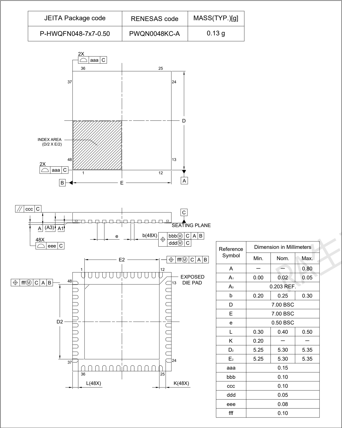
Figure 2.3 QFN 48-pin
