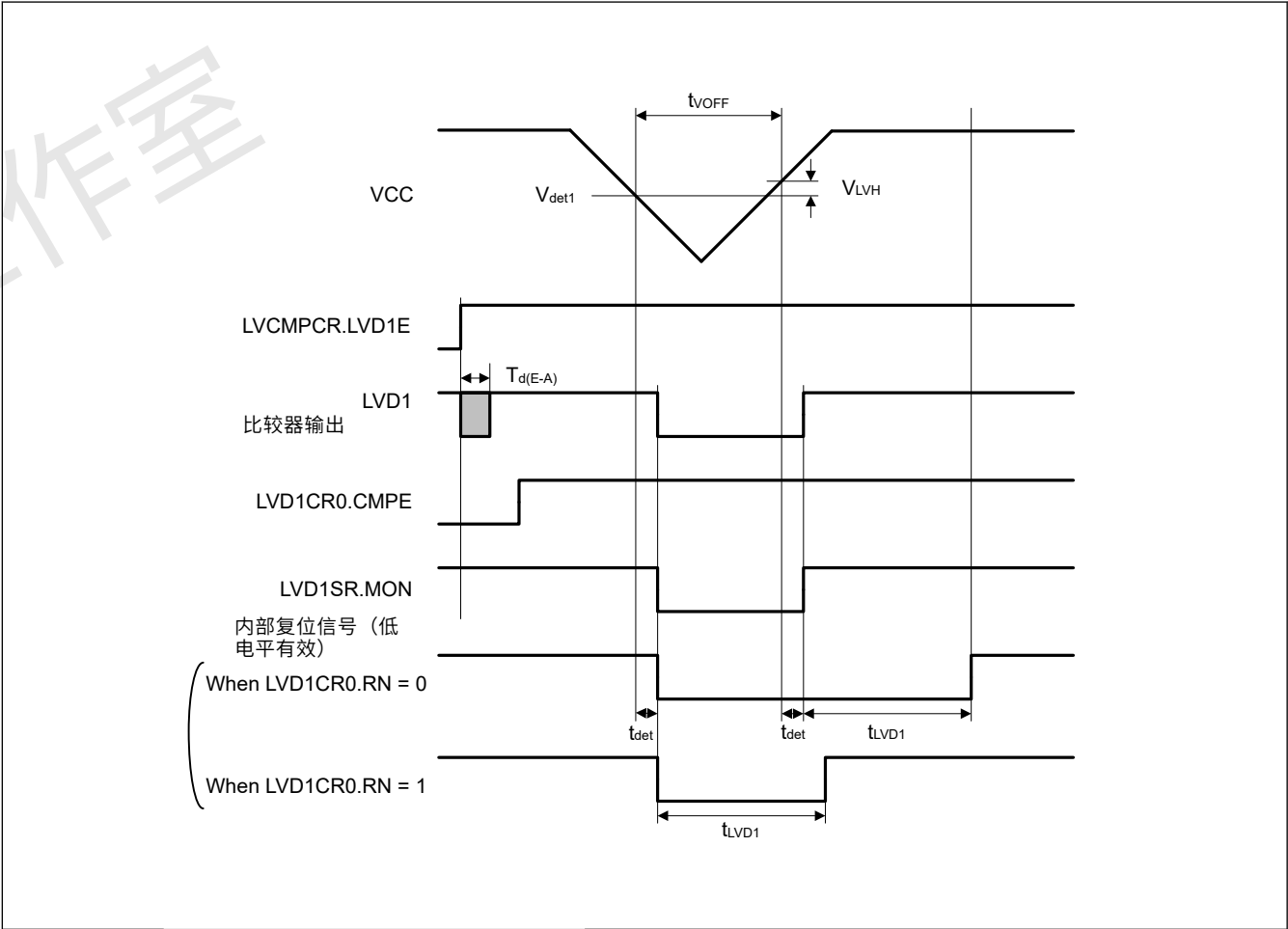
Figure 2.62 电压检测电路时序 (V det1 )
