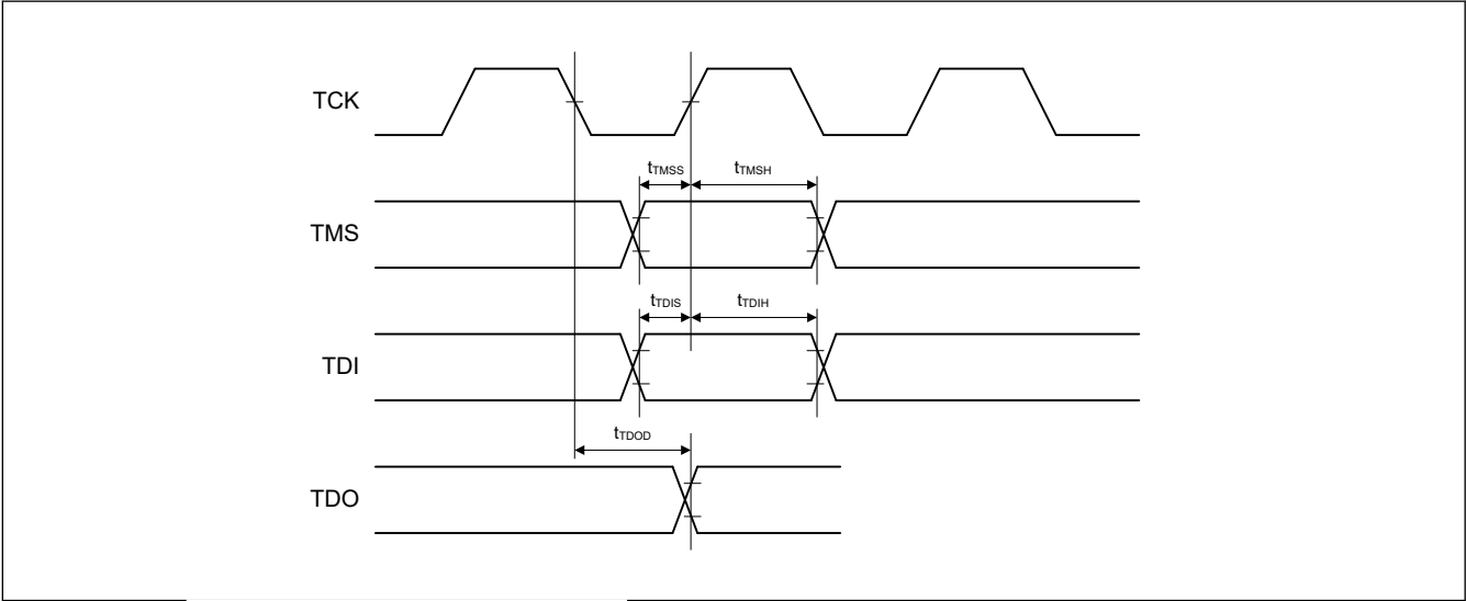
Figure 2.68 边界扫描输入输出时序
