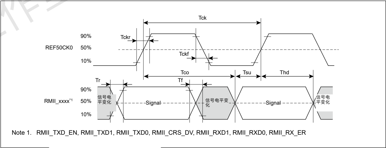
Figure 2.49 REF50CK0和RMII信号时序
