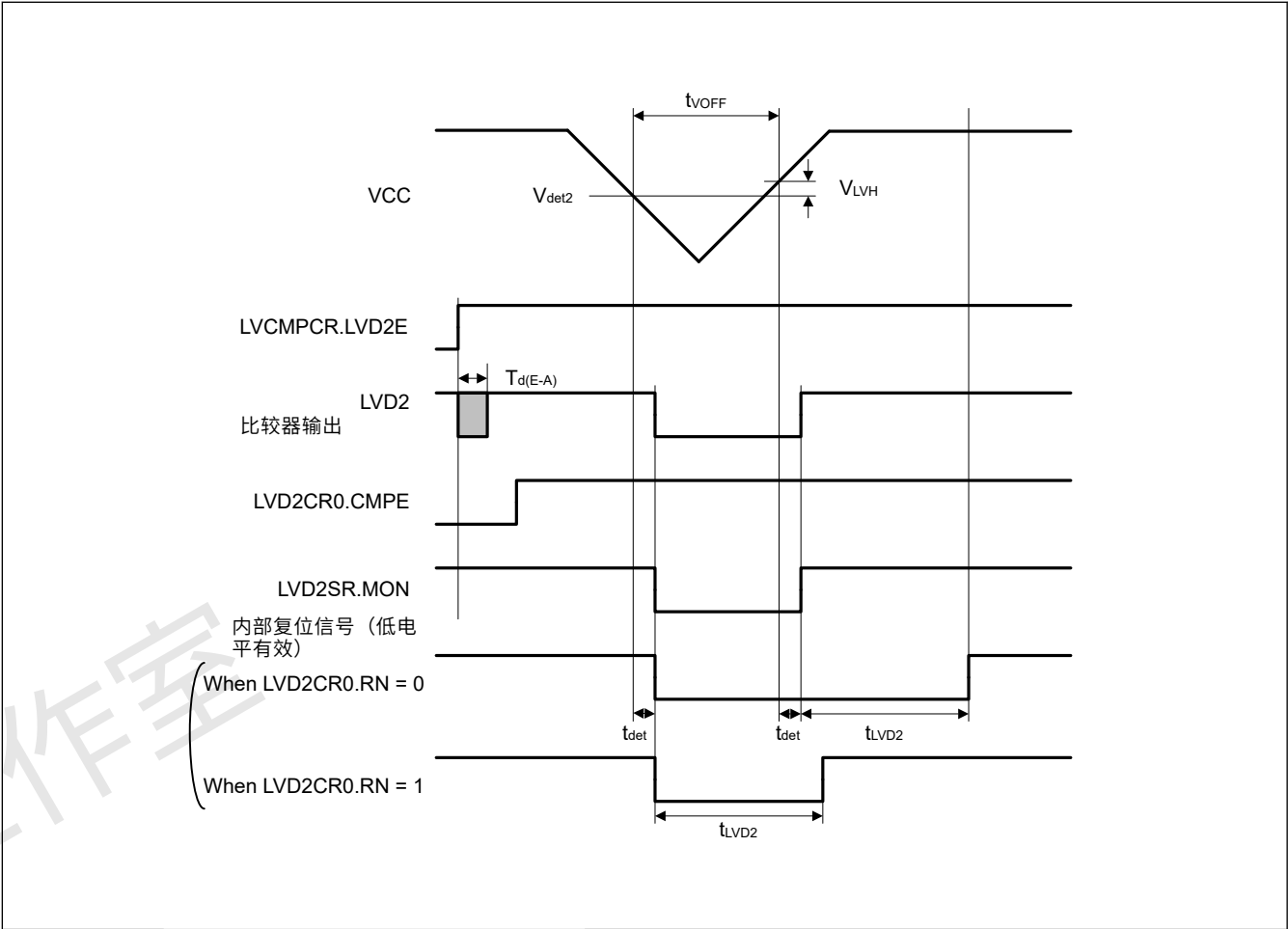
Figure 2.63 电压检测电路时序 ( V_{det2} )
