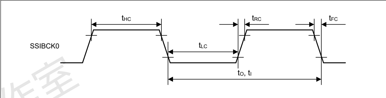
Figure 2.43 SSIE时钟输入输出时序
