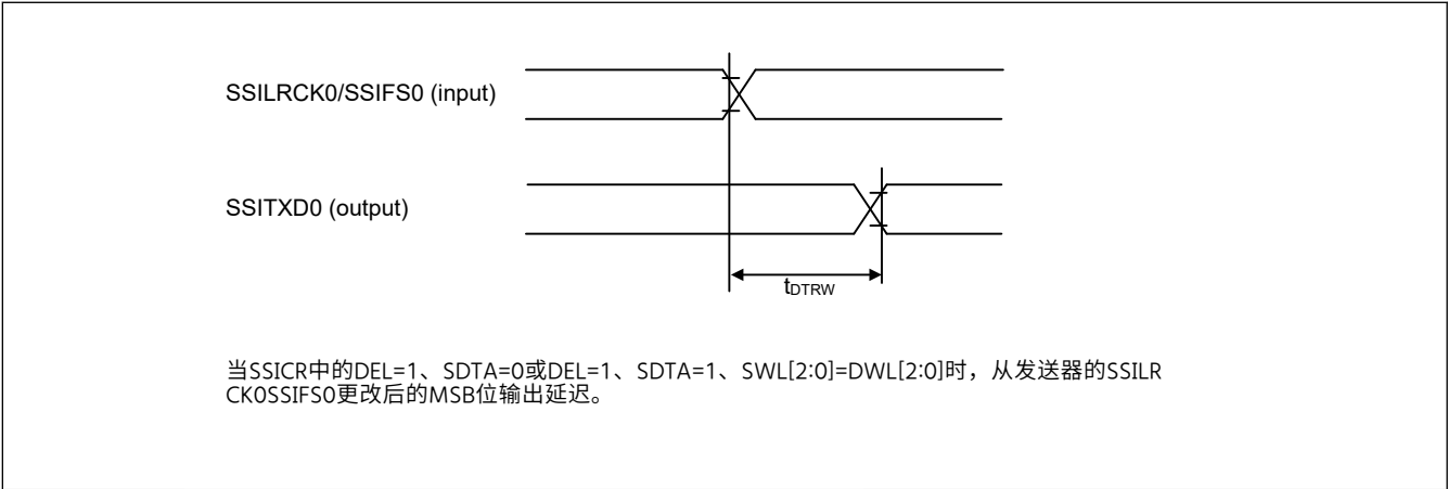
Figure 2.47 SSILRCK0SSIFS0更改后的SSIE数据输出延迟
