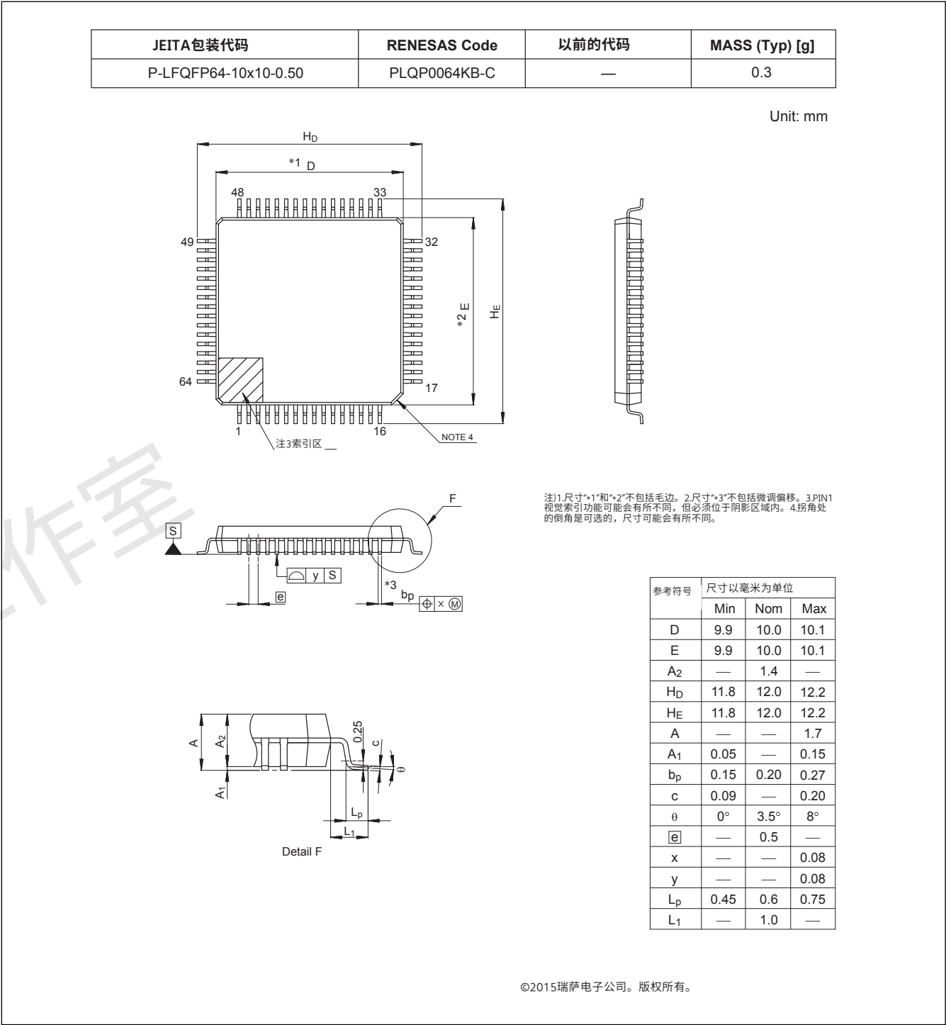
Figure 2.2 LQFP 64-pin
