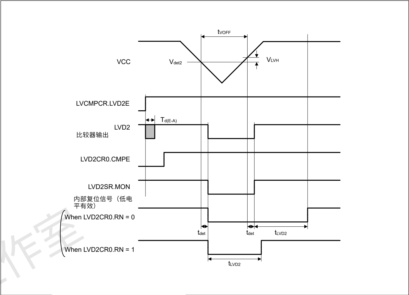
Figure 2.59 电压检测电路时序 (V det2 )
