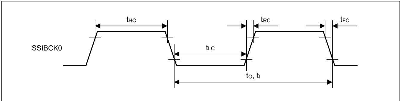
Figure 2.44 SSIE时钟输入输出时序
