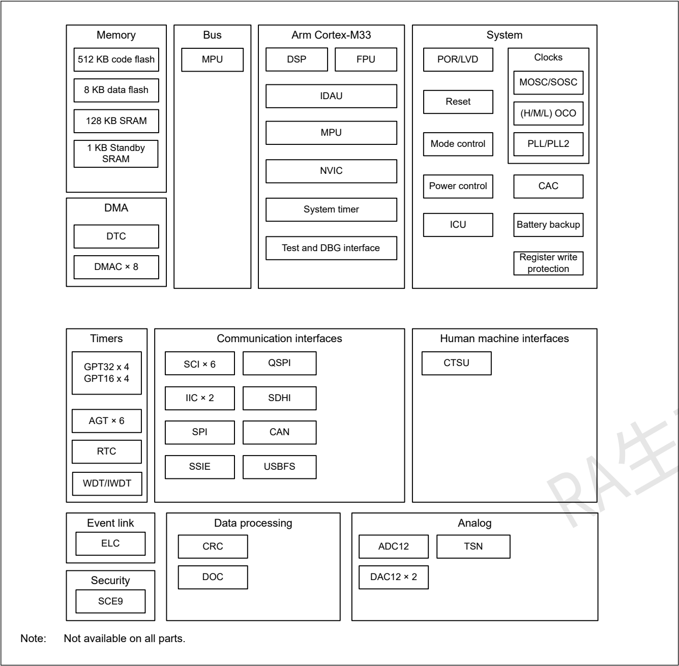
Figure 1.1 Block diagram
