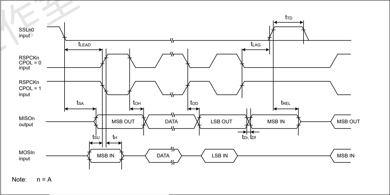
Figure 2.39 CPHA=0时从机的SPI时序
