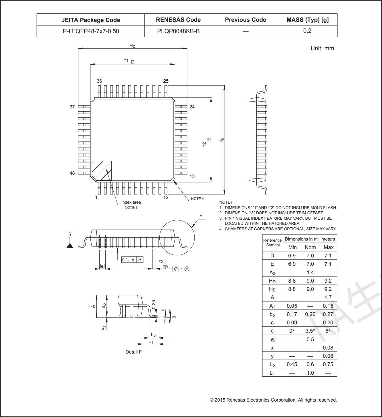
Figure 2.3 LQFP 48-pin
