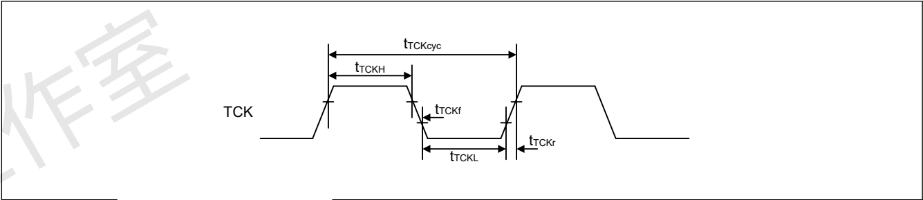
Figure 2.63 边界扫描TCK时序
