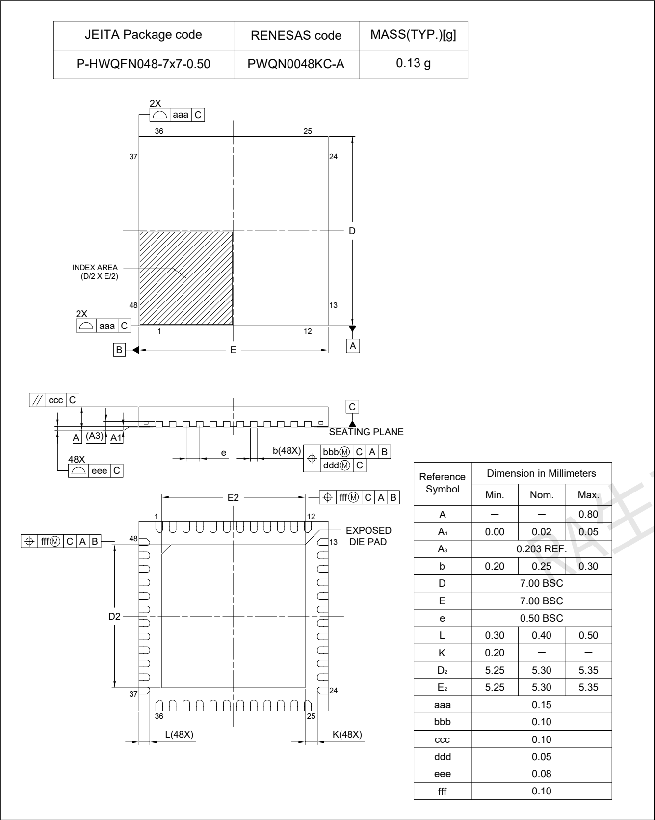
Figure 2.4 QFN 48-pin
