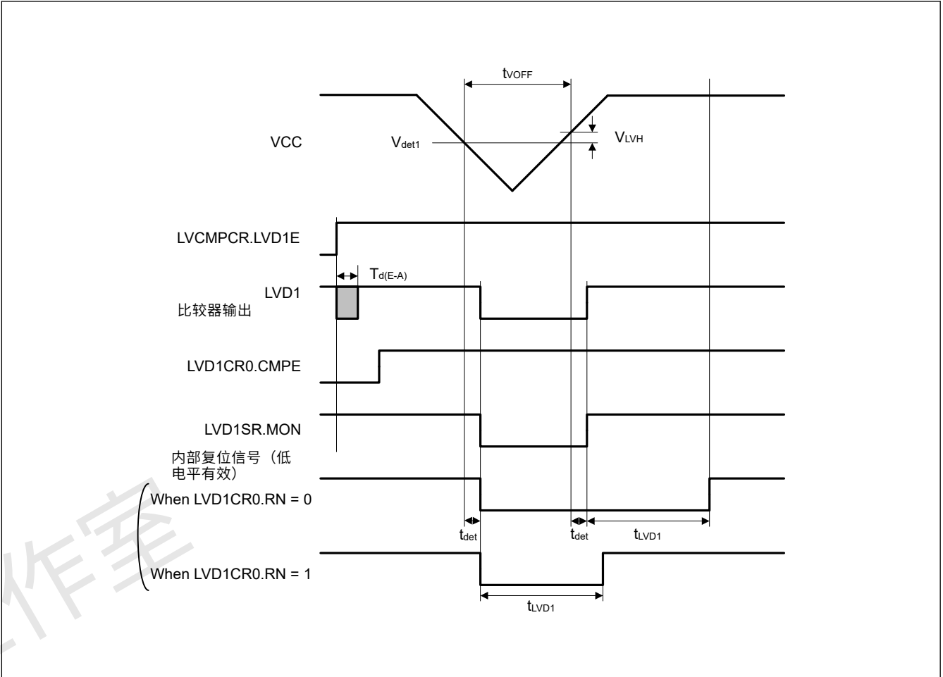
Figure 2.58 电压检测电路时序 ( V_{det1} )
