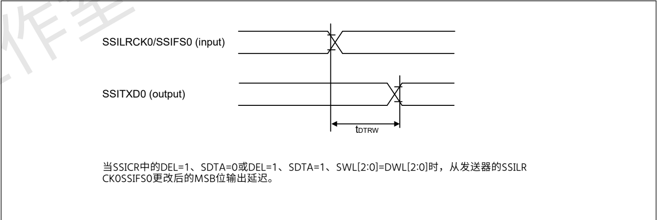
Figure 2.48 SSILRCK0SSIFS0更改后的SSIE数据输出延迟
