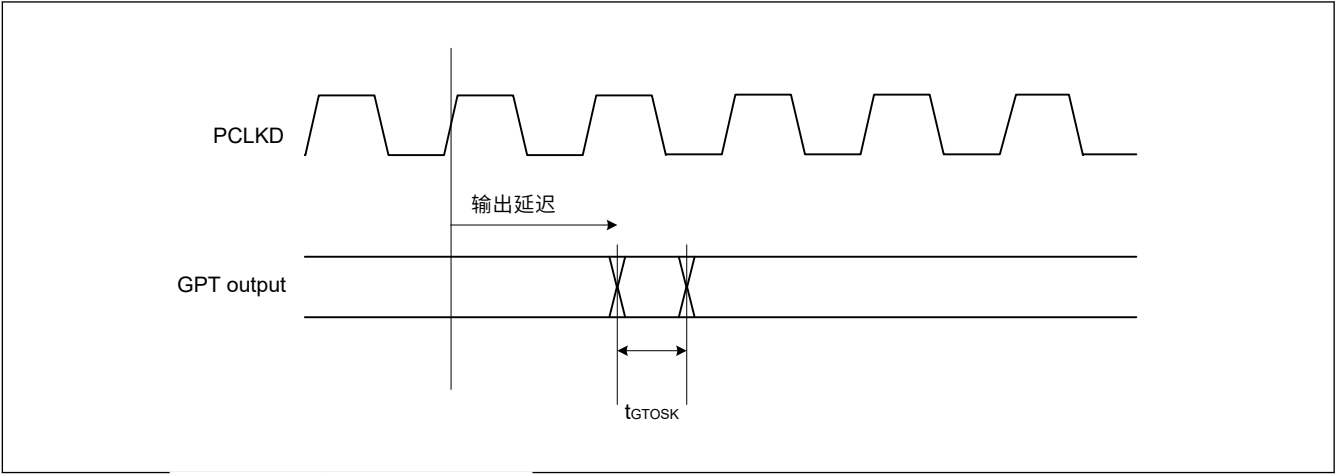
Figure 2.23 OPS的GPT输出延迟偏差
