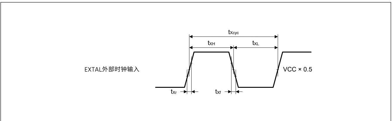
Figure 2.7 EXTAL外部时钟输入时序
