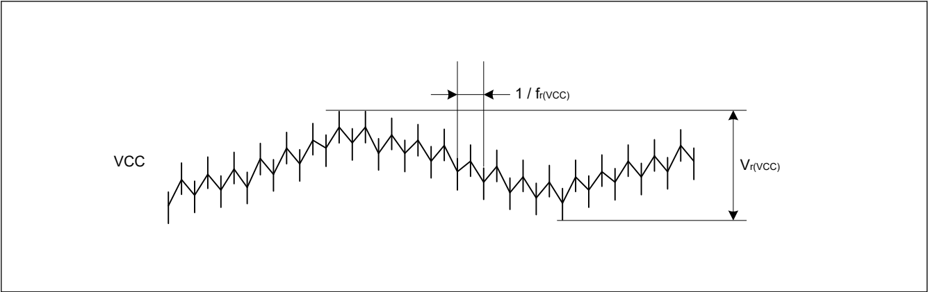
Figure 2.6 Ripple waveform
