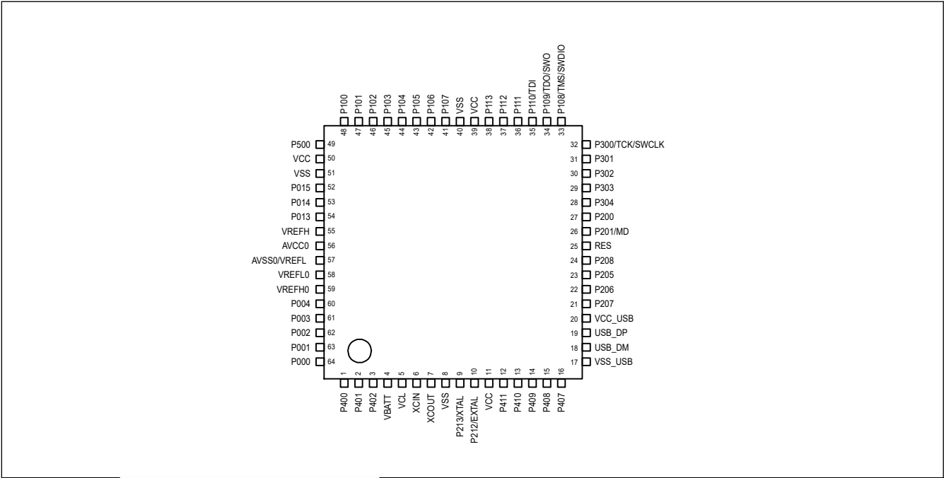
Figure 1.4 LQFP64引脚的引脚分配
