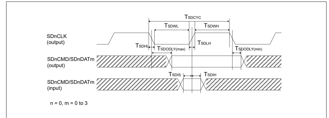
Figure 2.49 SDMMC主机接口信号时序
