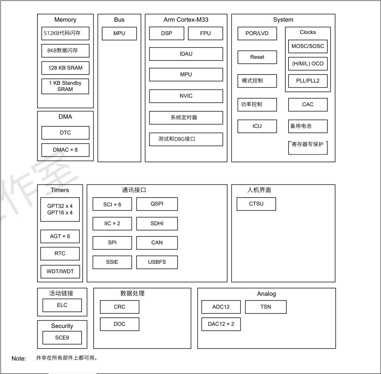
Figure 1.1 框图
