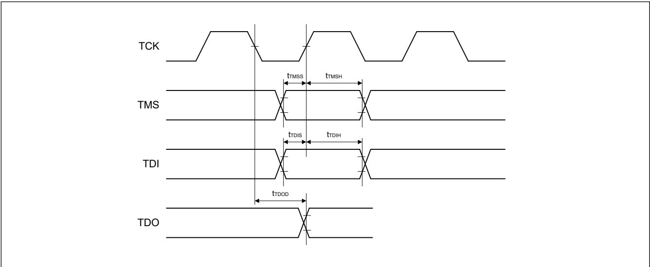
Figure 2.64 边界扫描输入输出时序
